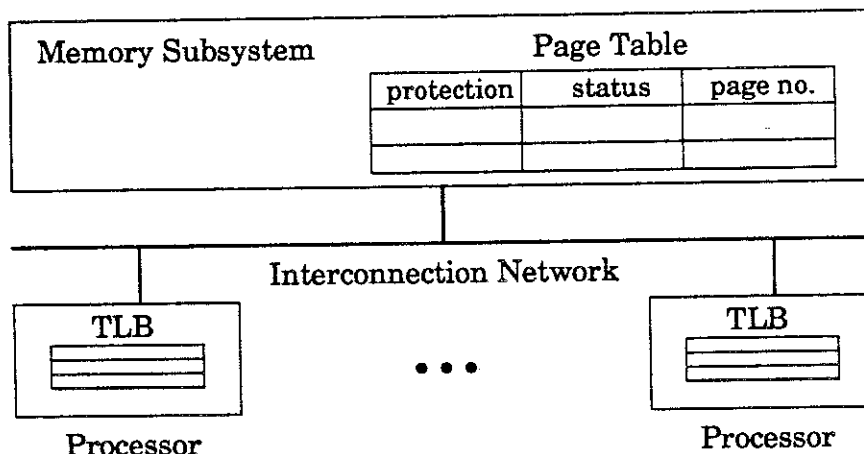
Figure 2.1. The model of a shared-memory multiprocessor.
