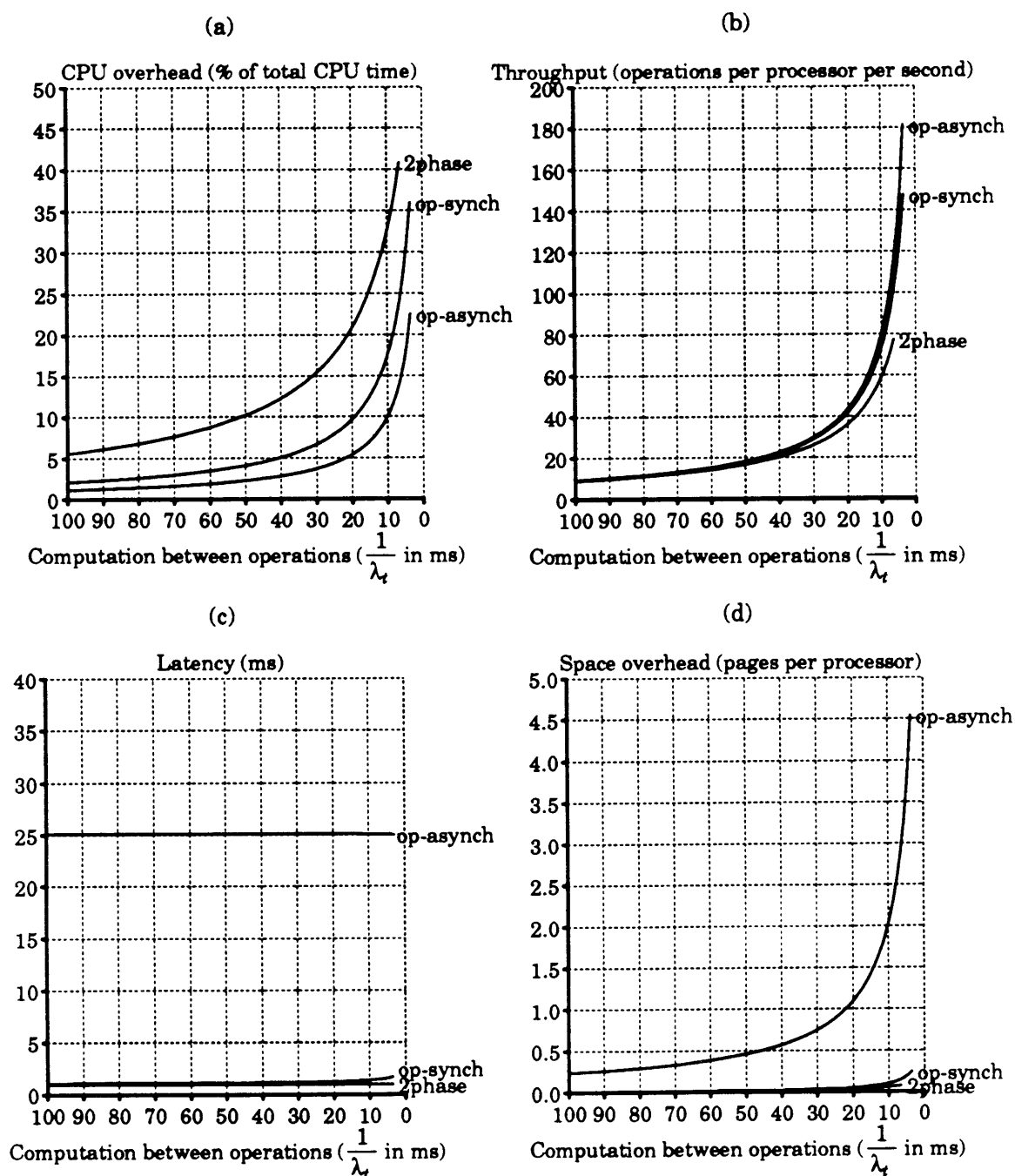
Figure 4.6. The effect of the request rate on performance. Parameters are M = 16 , \lambda_d = 100/\text{sec.} , X_d = 0.5 ms, X_i = X_{req_1} = X_{req_2} = X_{reply} = 0.04 ms, X_j = 25 ms, and p_0 = 0.0002 .
