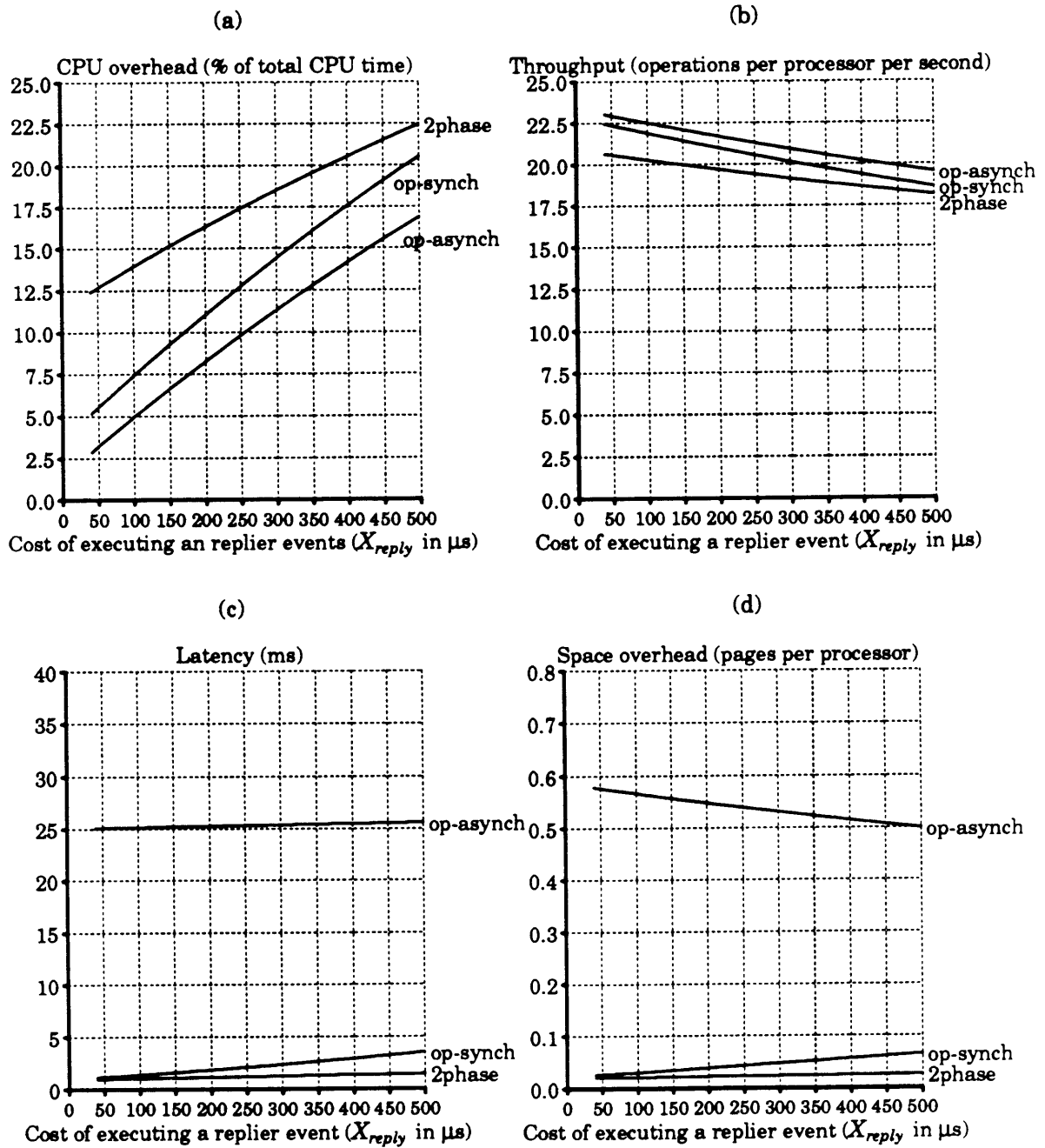
Figure 4.7. The effect of service time on performance. Parameters are M = 16 , \lambda_t = 25/\text{sec.} , \lambda_d = 100/\text{sec.} , X_d = 0.5 \text{ ms} , X_i = X_{req_1} = 0.04 \text{ ms} , X_{req_1} = X_{reply} , X_j = 25 \text{ ms} , and p_0 = 0.0002 .
