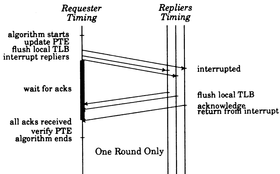
Figure 3.3. The optimistic algorithm. Only the requester blocks in the shaded interval.
