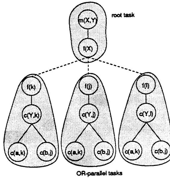
Figure 2.5: OR-Parallel Tree
