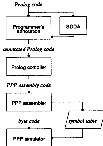
Figure 5.1: Program Transformation
