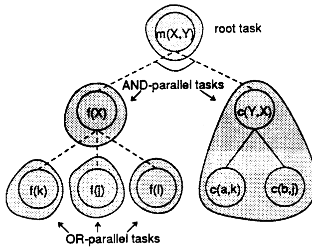
Figure 2.6: AND-OR Parallel Tree
