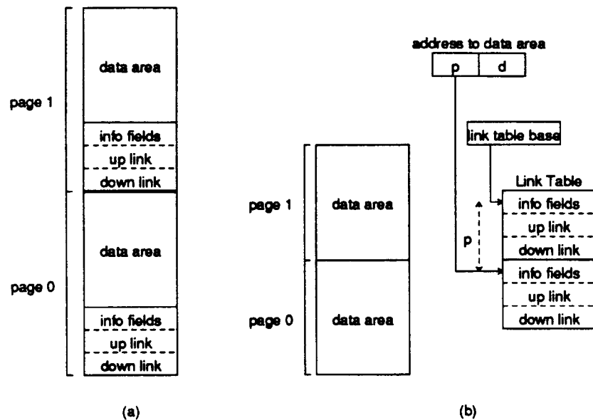
Figure 4.2: Two Link Storage Schemes for ELPS
