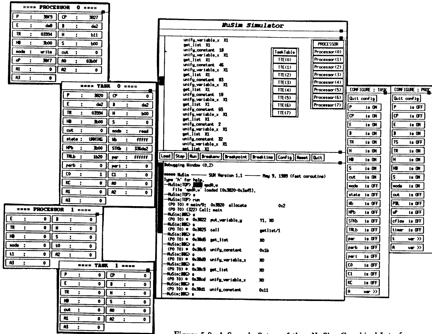
Figure 5.8: A Sample Setup of the xNuSim Graphical Interface
