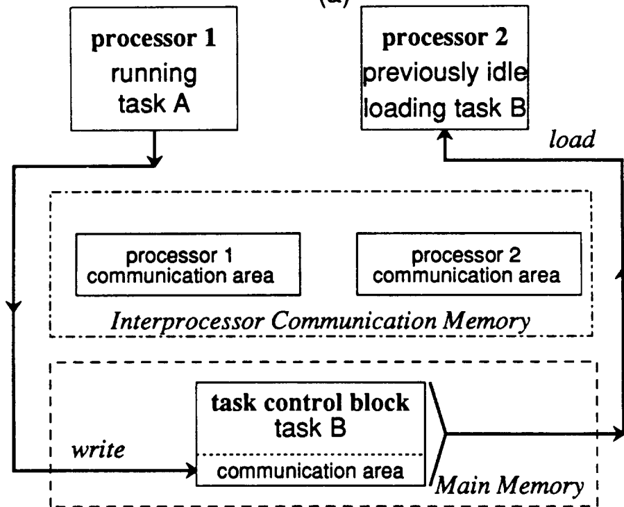
Figure 5.3: Task Communication
