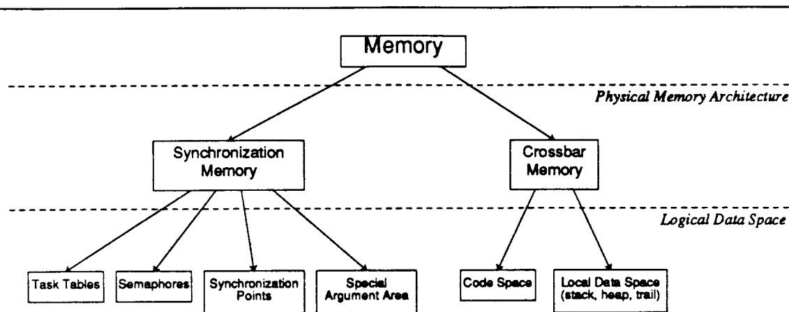
Figure 8.3: Mapping of the PPP Storage Model onto the Two-Tier Memory System
