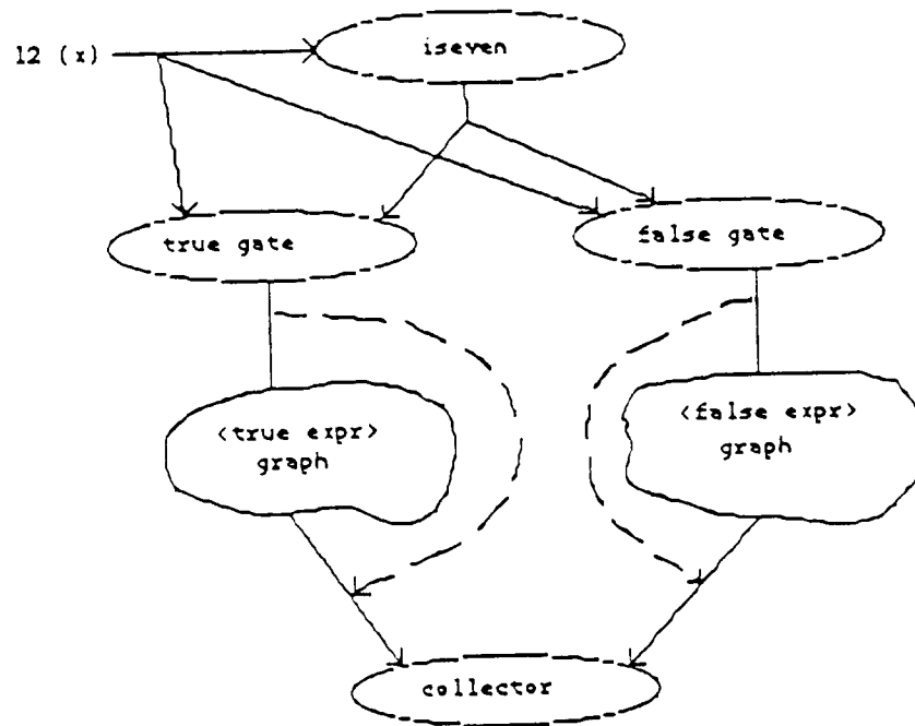
Figure 4: Conditional Statement
