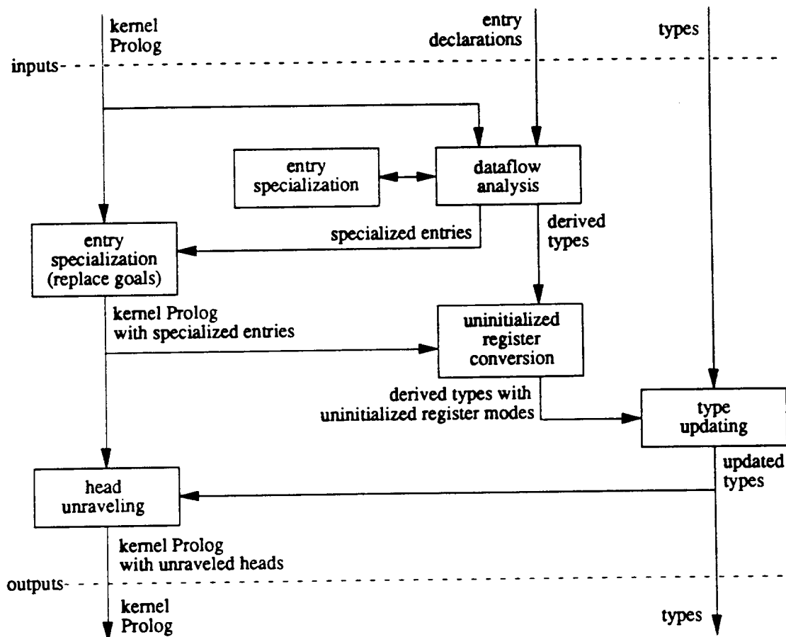
Figure 4.9 – Integrating analysis into the compiler
