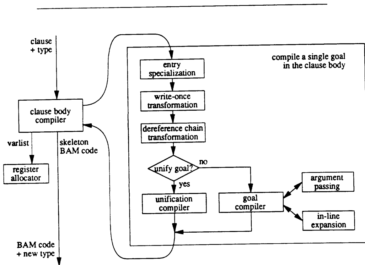
Figure 5.1 – Structure of the clause compiler
