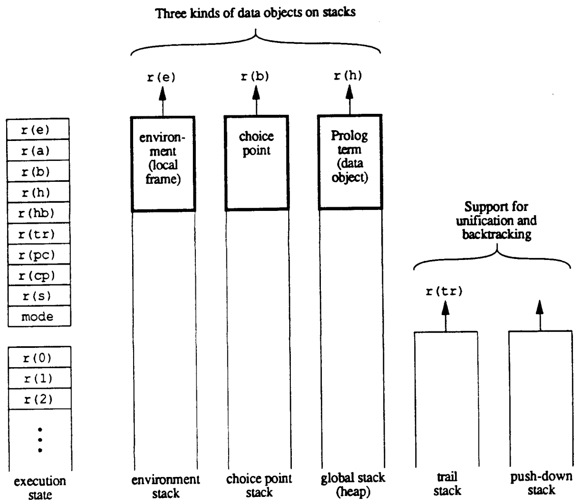
Figure 2.6 – Data structures of WAM and BAM
