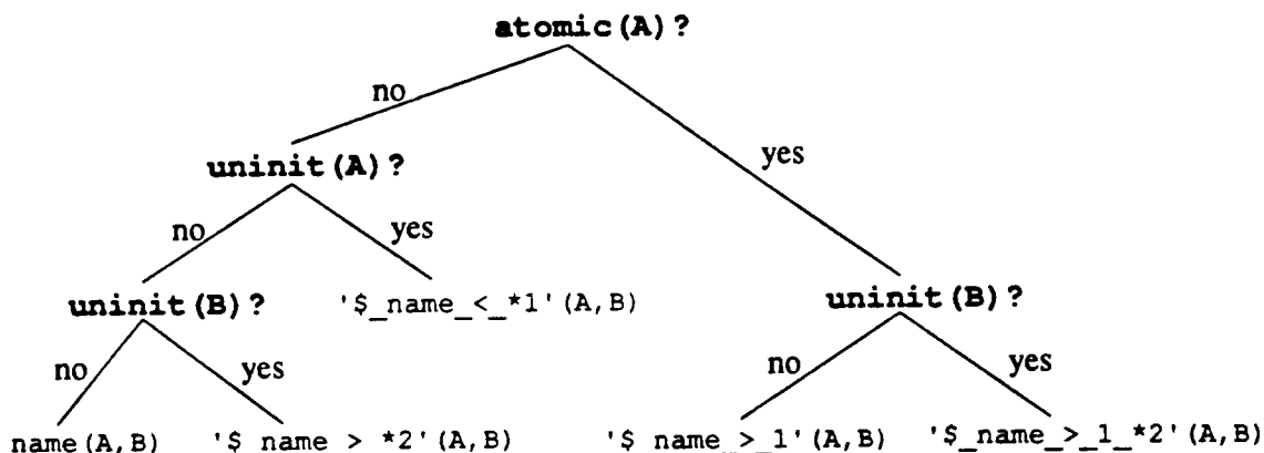
Figure 5.6: Example of a modal entry tree for entry specialization
