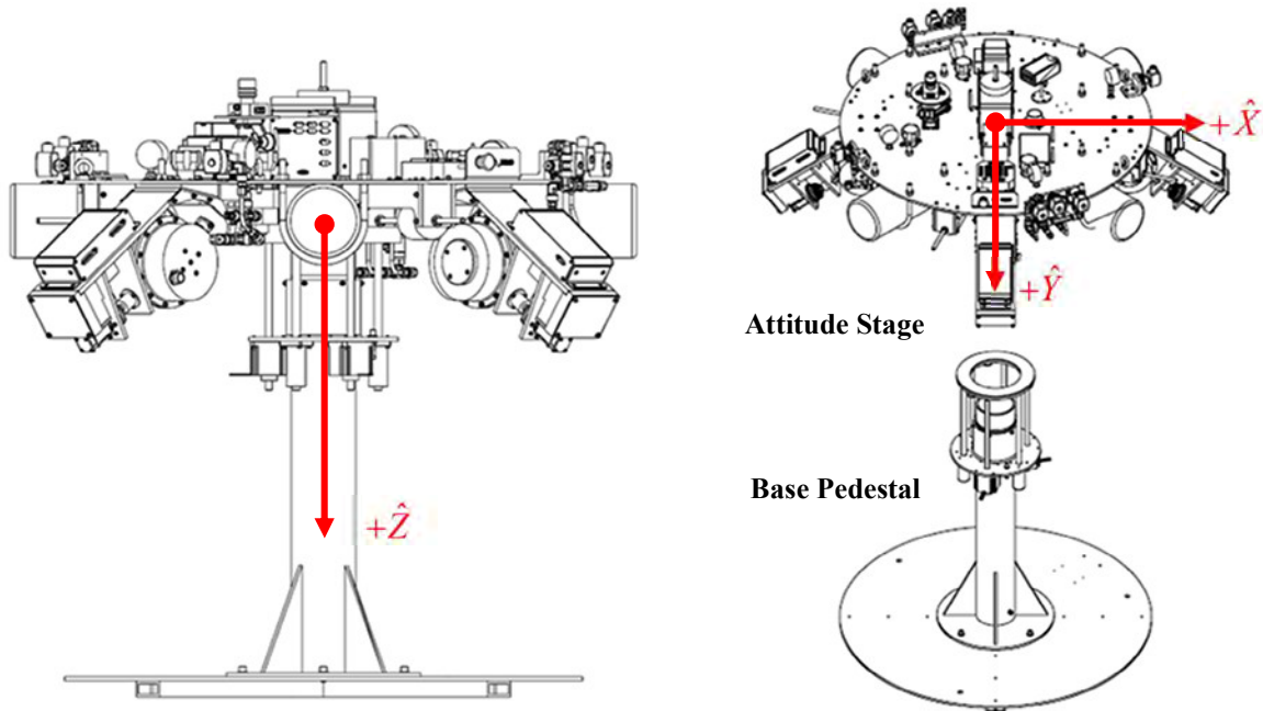
Figure 3. Overview of Andrews Space 3DOF Satellite Simulator
