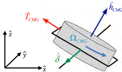
Figure 2. CMG torque and angular momentum vectors
