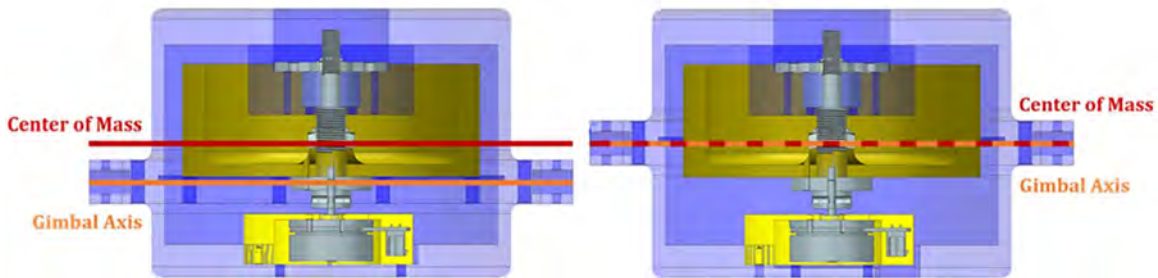
Figure 14. Side-by-side comparison of previous and updated momentum wheel case designs
