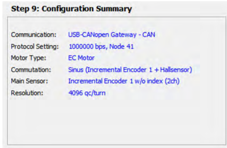
Figure 66. Gimbal motor setup (Step 9)
