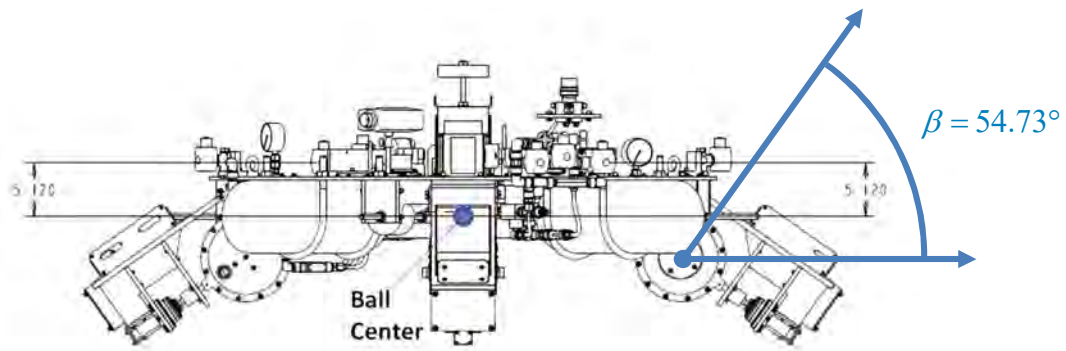
Figure 7. Side view of NPS R-SAT simulator
