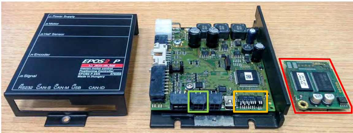
Figure 20. Maxon EPOS2 P 24/5 motor controller with PLC module removed
