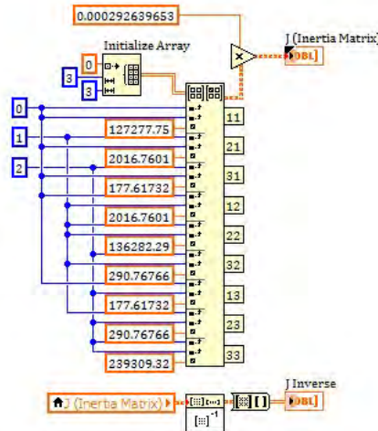
Figure 32. Inertia matrix generation in CMG Flight Computer.vi
