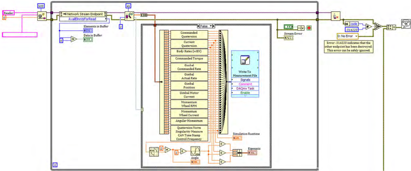
Figure 37. Data acquisition logic in Reader VI.vi
