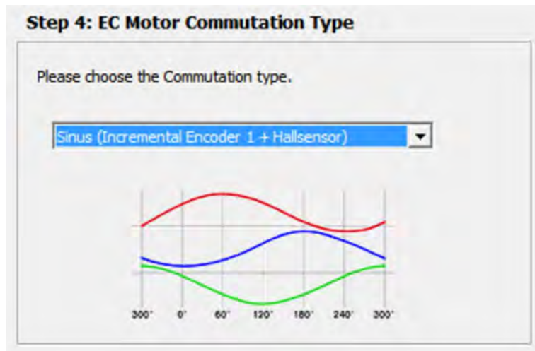
Figure 61. Gimbal motor setup (Step 4)
