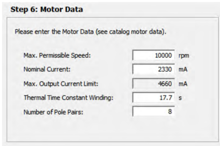
Figure 71. Momentum wheel motor setup (Step 6)
