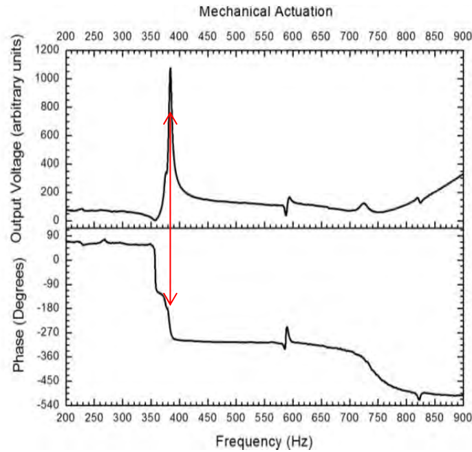
Figure 7. Household Vibrational Testing Results
