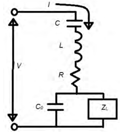
Figure 3. Equivalent Electrical Circuit of Piezoelectric Energy Harvester
