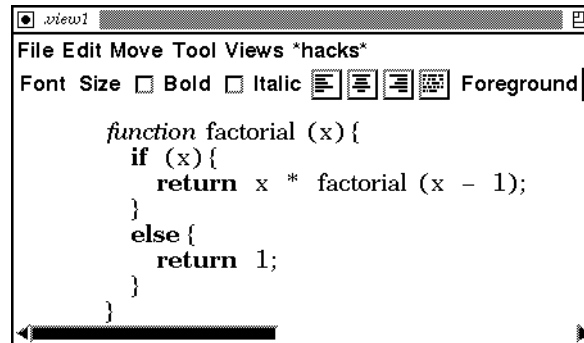
Figure A.2: An alternate presentation of the factorial example in which the left brace beginning each block is placed at the end of the line containing the preceding material.
