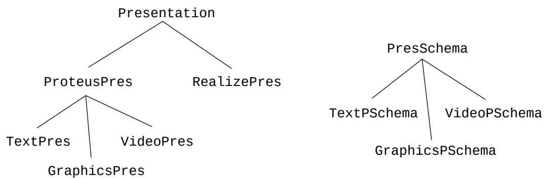
Figure 5.2: The two C++ class hierarchies that implement the kernel/shell architecture of Proteus.
