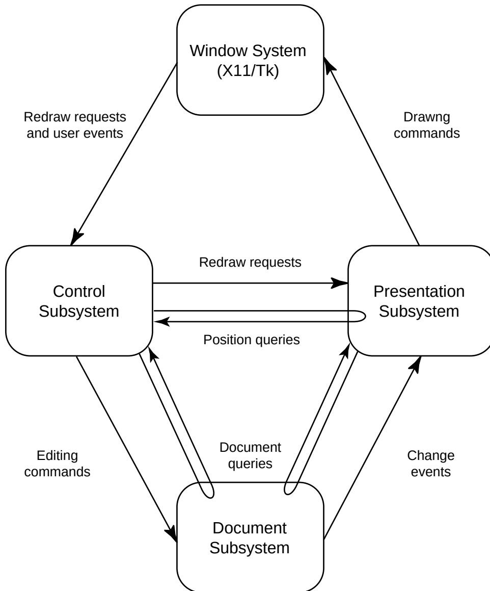
Figure 3.1: Overview of Ensemble's architecture. Single-headed arrows represent commands. U-shaped arrows represent query-and-response interactions.
