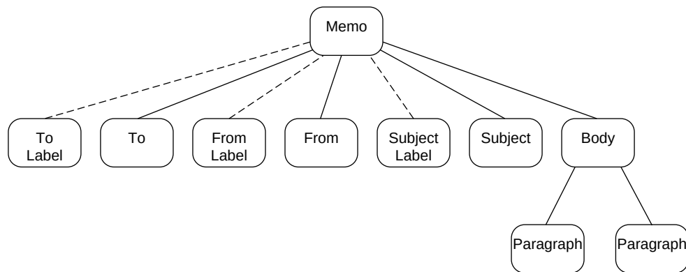
Figure 4.11: The presentation tree for the memorandum example. Arcs that are present in both the document and presentation trees are solid. Arcs that are only found in the presentation tree are dashed.
