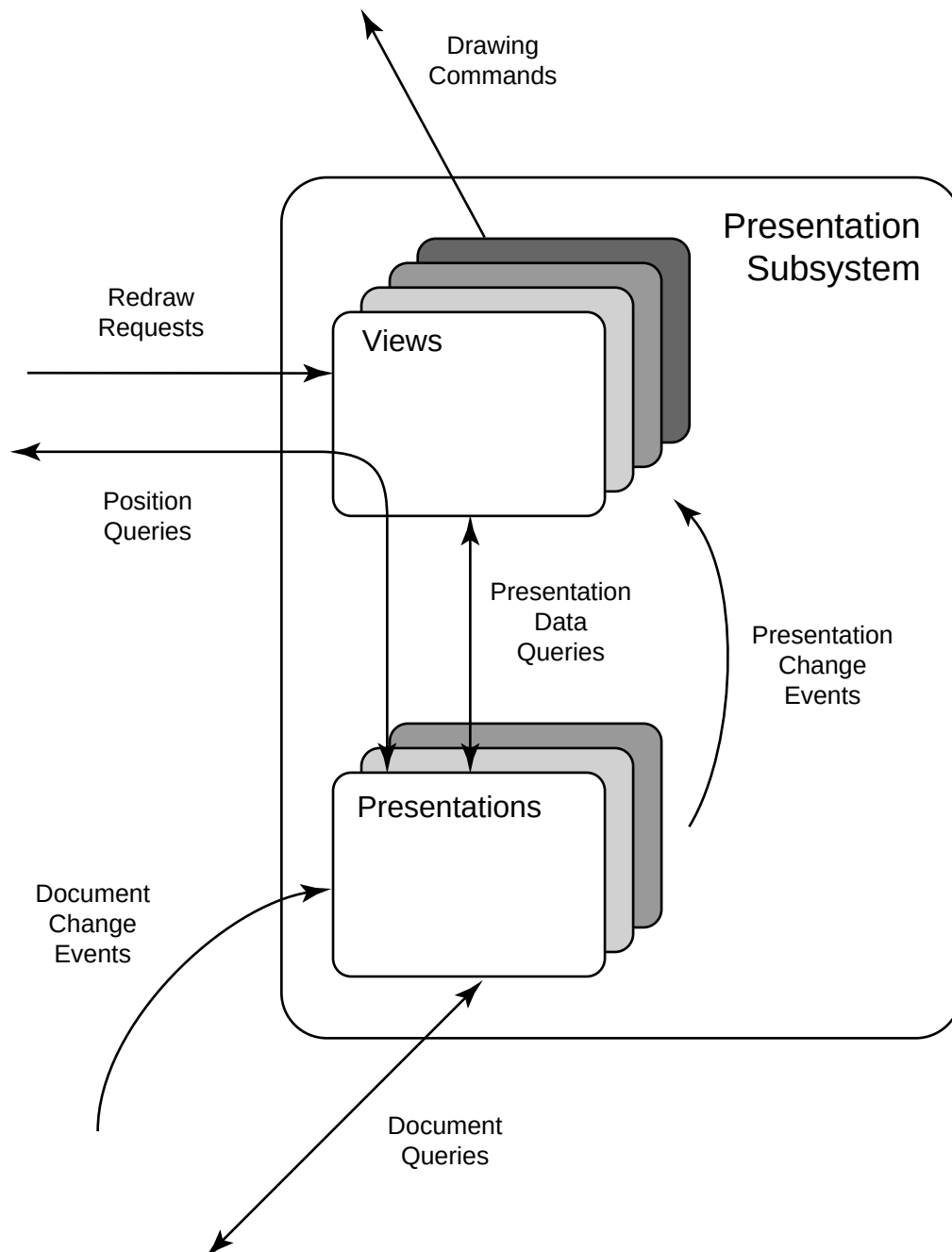
Figure 4.3: Information flow within Ensemble's presentation subsystem. Single-pointed arrows represent commands. Double-pointed arrows represent call-and-return interactions. Proteus is not shown.
