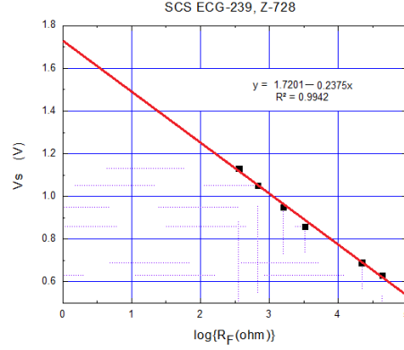
Figure 12. Switching Voltage as a Function of R_F
