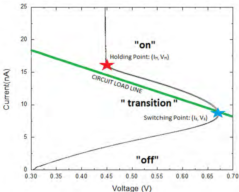
Figure 6. SCS (ECG-239) Standalone I-V Characteristic with Added Circuit Load Line
