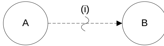
Figure 5. Cancelling an Edge (from Buss, 2011)
