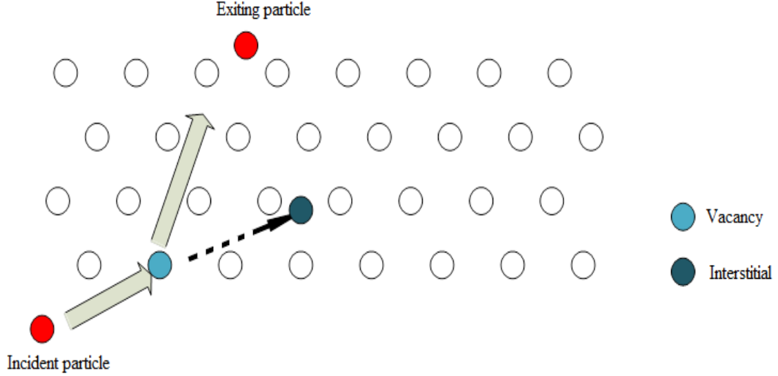
Figure 4. Displacement-damage due to radiation results in a Frenkel pair, vacancy and interstitial atom.
