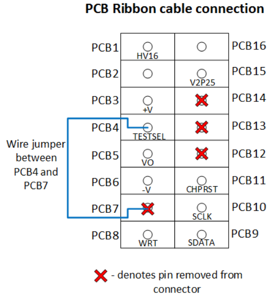
Figure 23 PCB ribbon cable connection.
