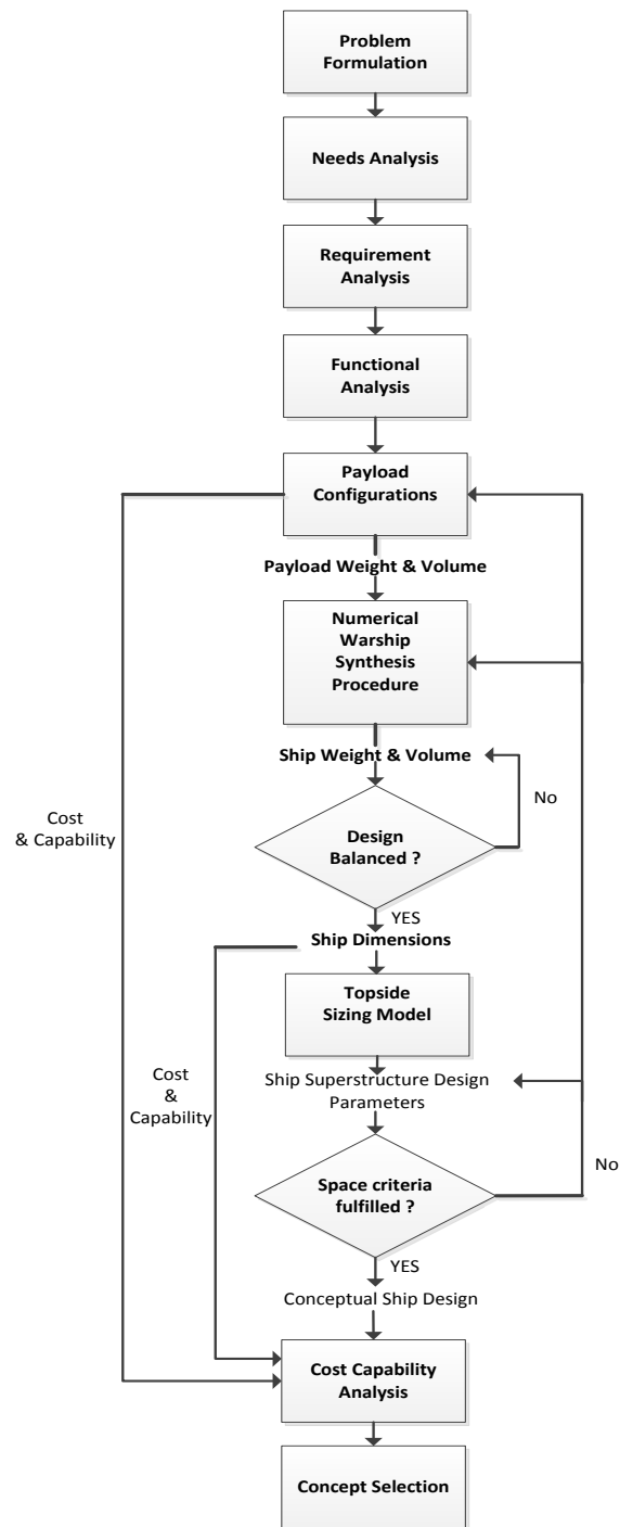
Figure 1. Overview of Systems Engineering Approach
