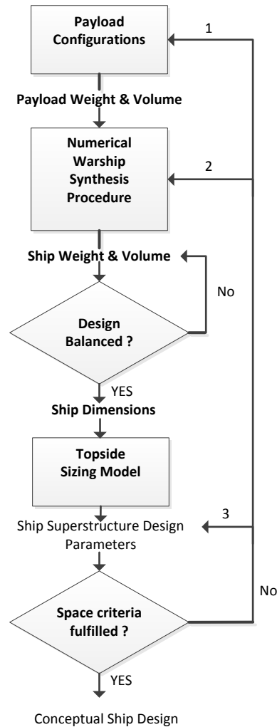
Figure 6. Design Methodology for Conceptual Ship Design
