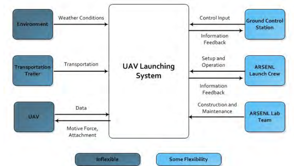
Figure 2.4: Launcher Context Diagram
