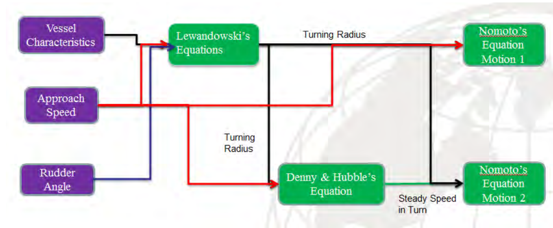
Figure 38. The Basic Diagram of the Mathematical Model
