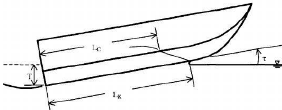
Figure 26. L_k and L_c of the Vessel, from [6]
