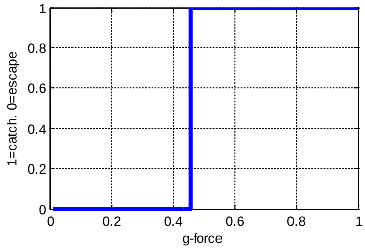
Figure 71. Catch/Escape Conditions vs. g-force in Pursuit Attack
