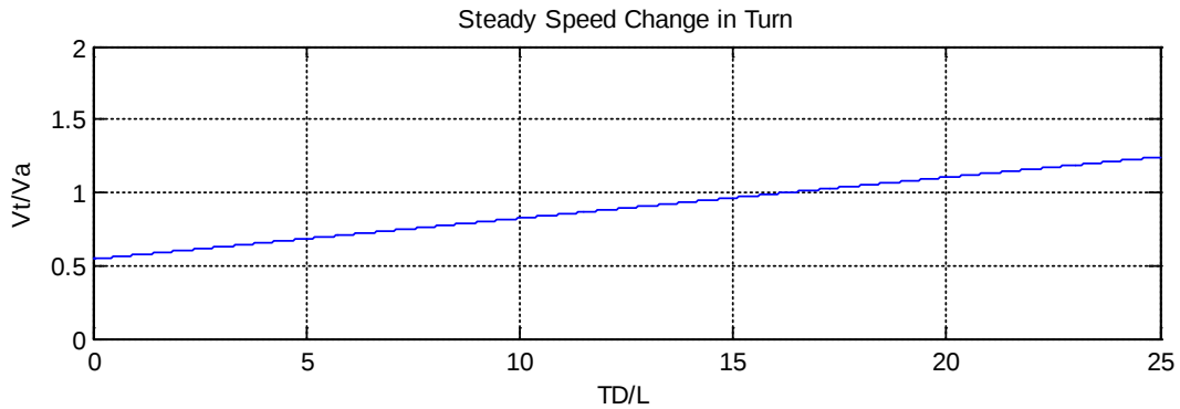
Figure 19. Turning Speed Ratio vs. Normalized Turning Diameter
