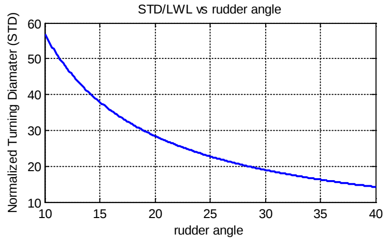
Figure 33. Normalized Turning Diameter vs. Rudder Angle for MRTP 16 Fast Intervention Craft
