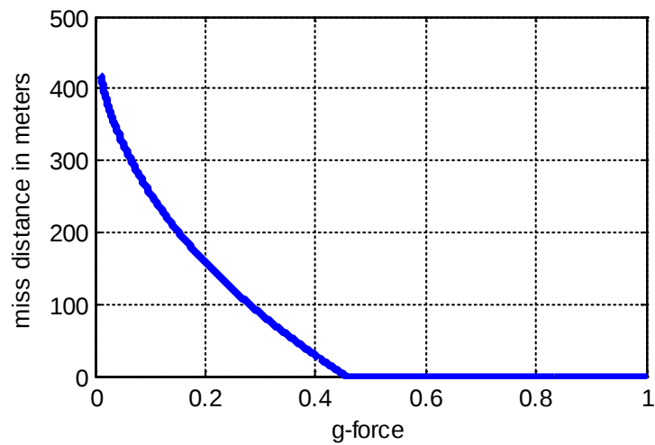
Figure 78. Miss Distances vs. g-force in Head-to-Head Situation
