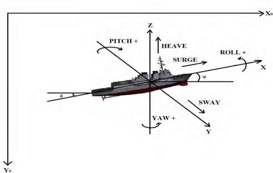
Figure 9. The Earth-Fixed Coordinate System and The Body-Fixed Coordinate System, from [11]
