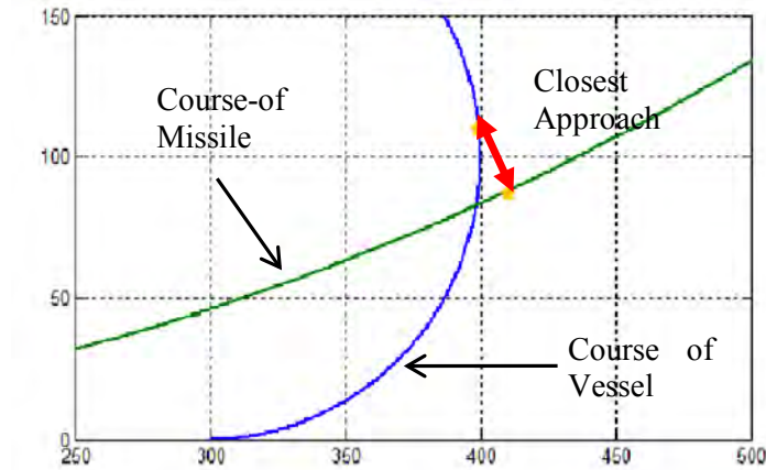
Figure 55. Closest Approach Illustration in Pursuit Attack
