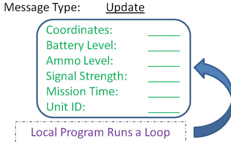
Figure 26. An in depth example of potential ROS message content.
