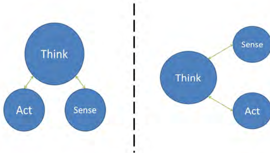
Figure 24. Typical architecture of a ROS program or network versus how it was implemented for this research.
