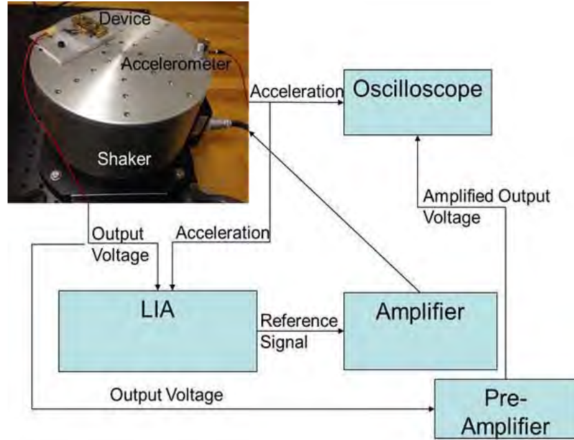
Figure 2. Vibrational test setup, from [1]
