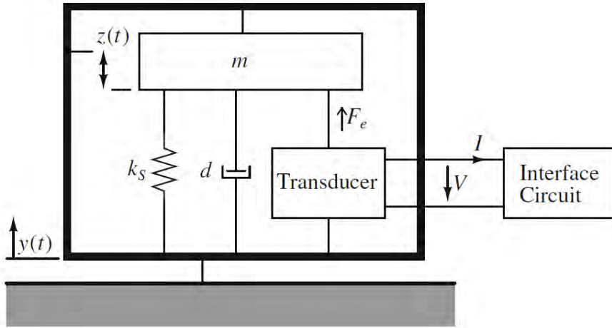
Figure 3. Mechanical equivalent model of a PEH, from [3]
