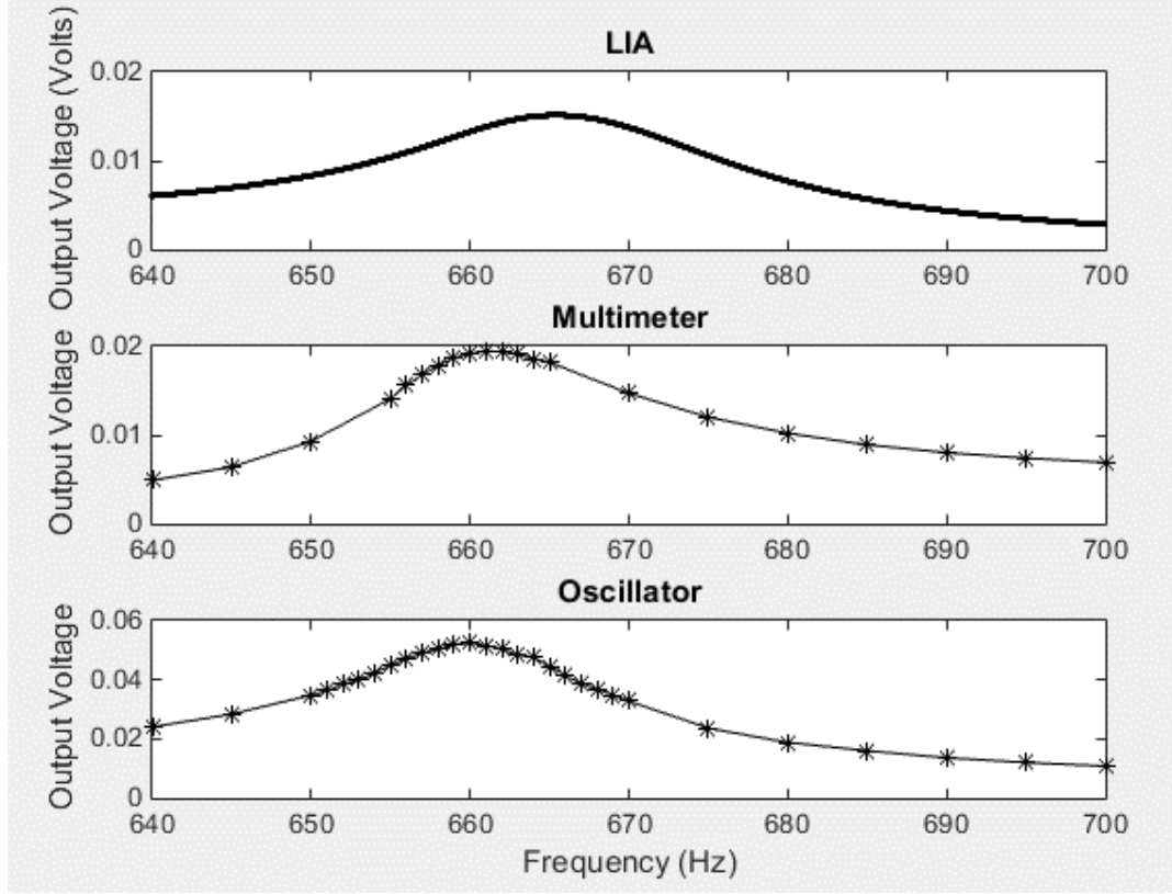
Figure 9. Measured output voltage for frequency sweep from 640 Hz to 700 Hz by LIA, multimeter, and oscilloscope
