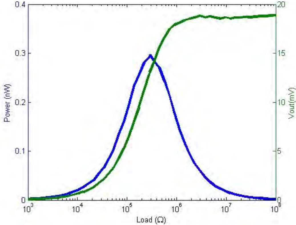
Figure 20. Power and output voltage under different loads
