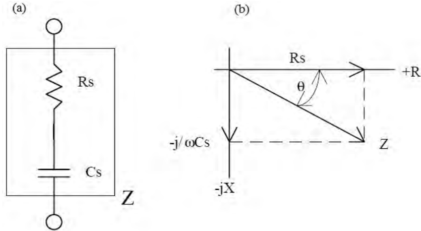
Figure 12. Series circuit for capacitive impedance (a) and phase diagram of impedance (b), from [6]
