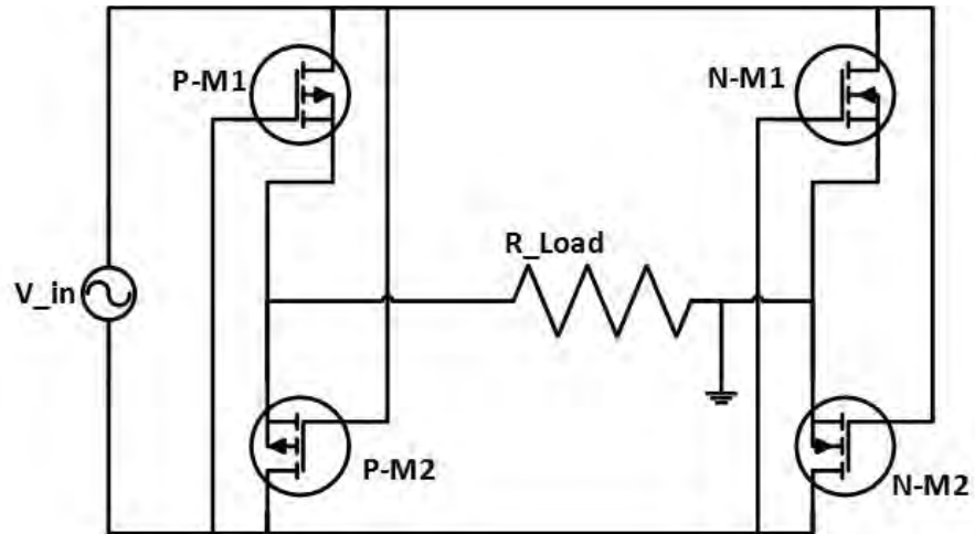
Figure 18. Full-wave passive MOSFET rectifier circuit, from [14]
