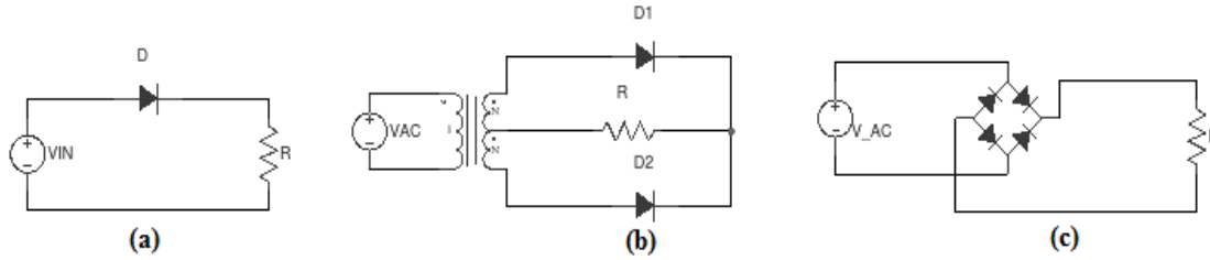
Figure 17. Half-wave rectifier (a), full-wave rectifier (b) and full-wave bridge rectifier (c) circuits
