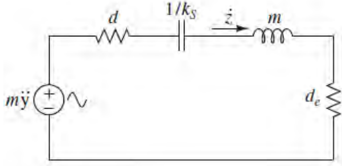
Figure 4. Electrical equivalent model of a PEH as an RLC circuit, from [3]
