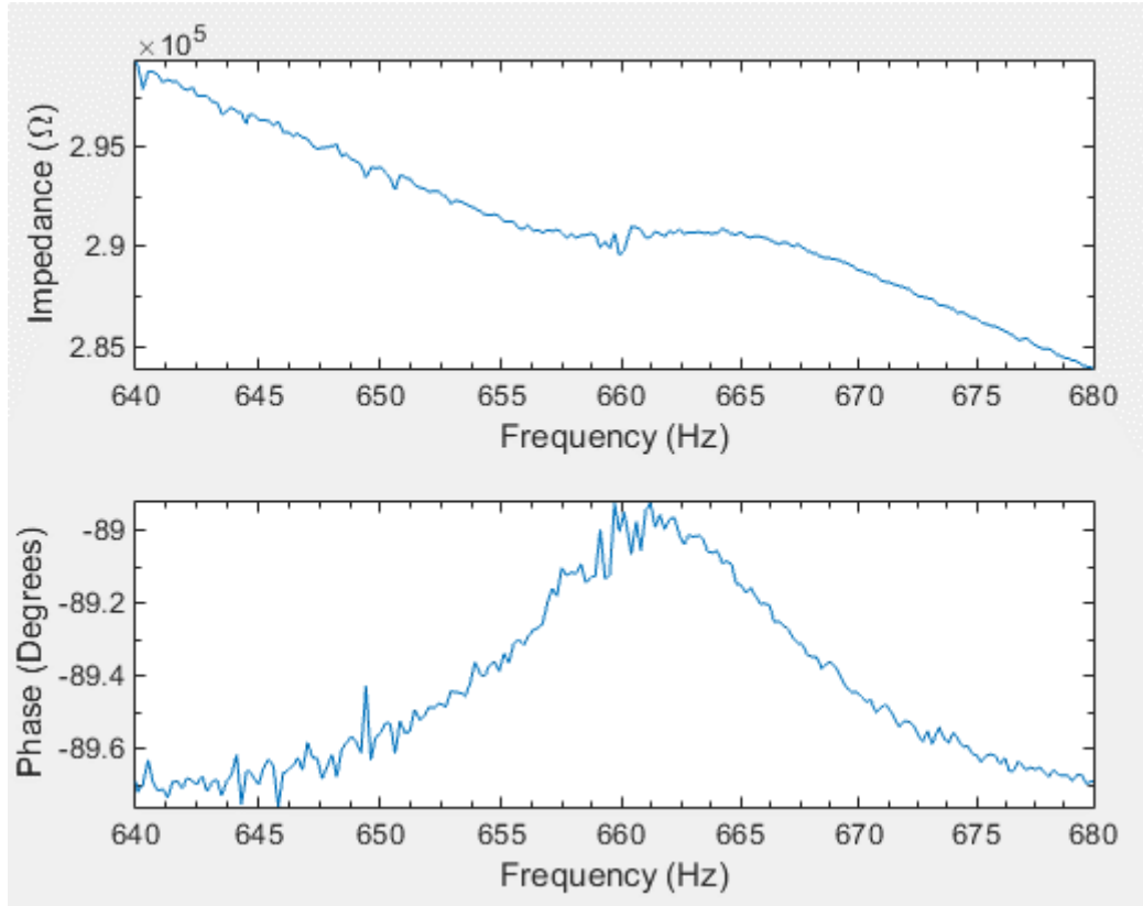
Figure 10. Impedance and phase angle of the device
