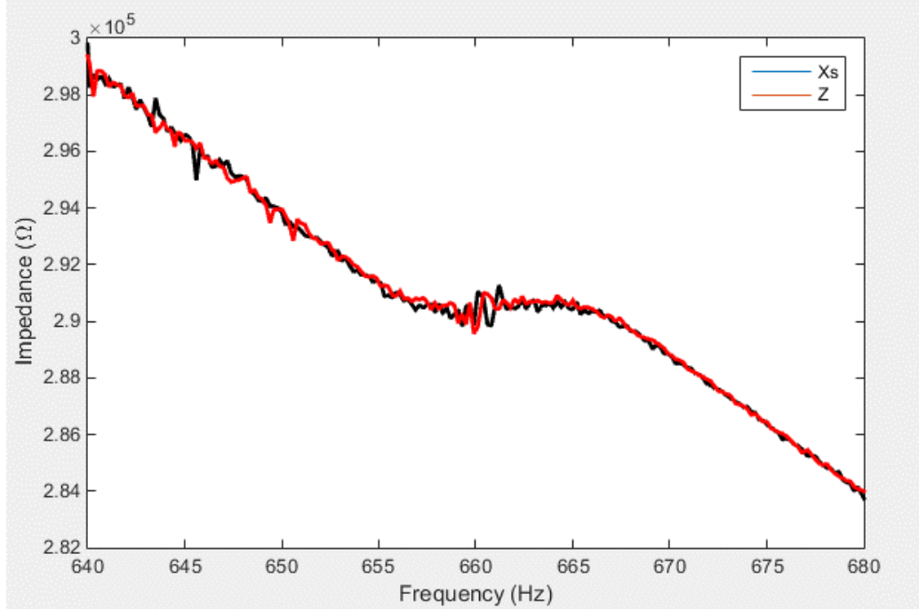
Figure 14. Impedance (Z) and reactance (Xs) of PEH
