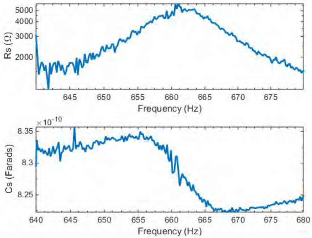
Figure 13. Resistance ( R_s ) and capacitance ( C_s ) of PEH
