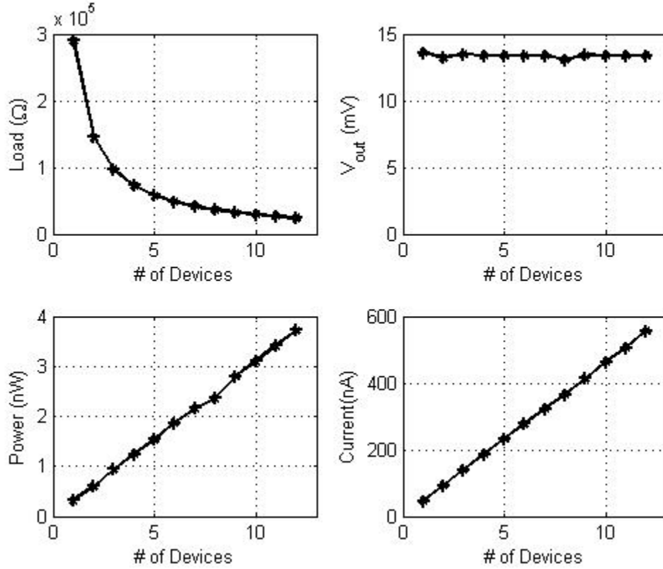
Figure 22. Matched load, output voltage, power, and current of devices connected in parallel
