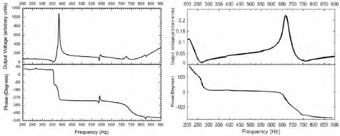
Figure 8. Normalized voltage output and phase of first (left) and second (right) devices
