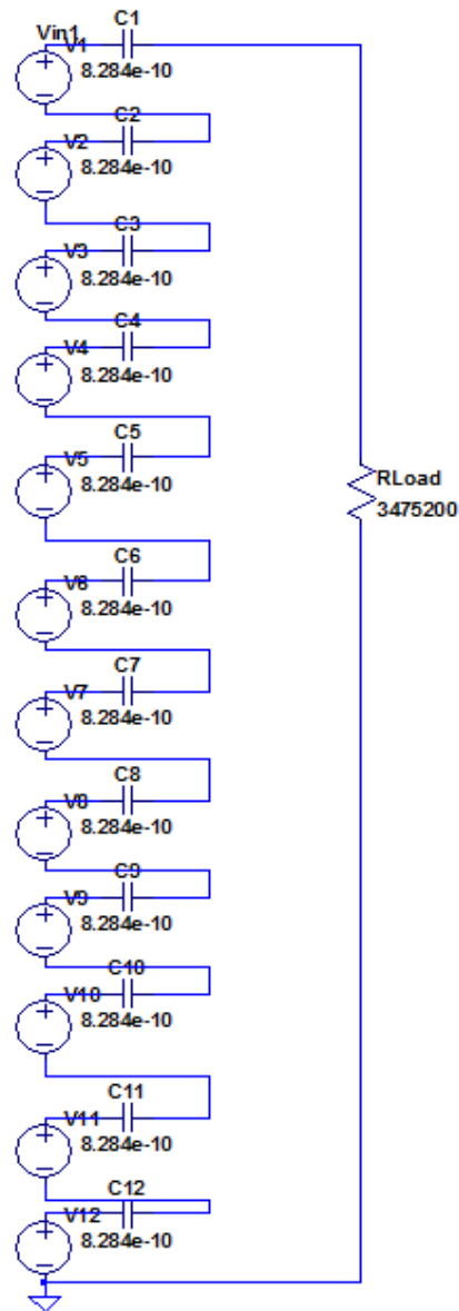
Figure 23. Twelve PEHs connected in series
