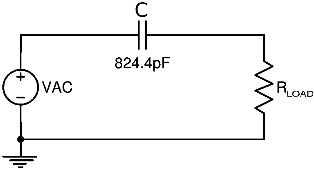
Figure 19. PSPICE model of the PEH
