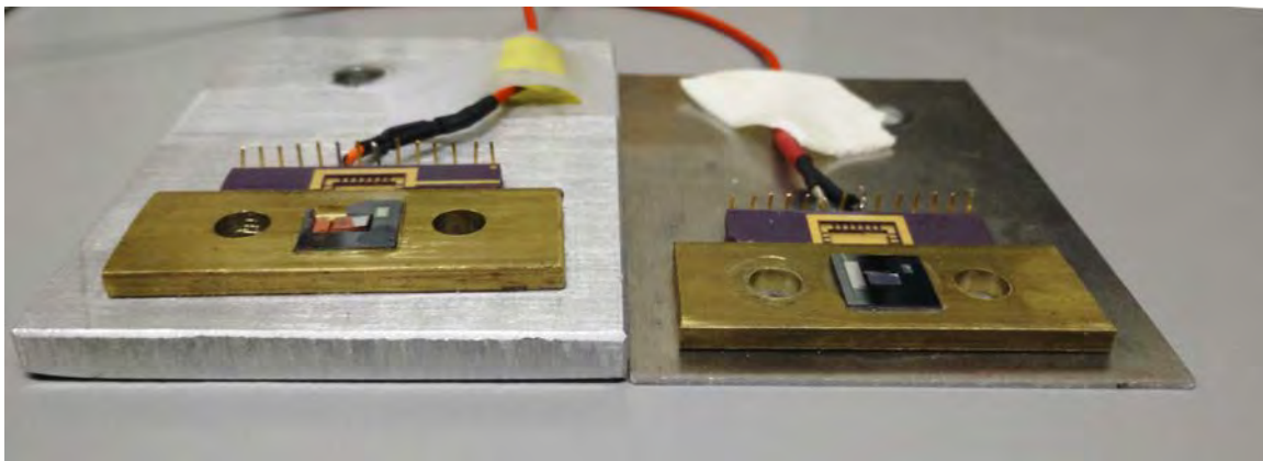
Figure 7. First (left) and second (right) PEHs
