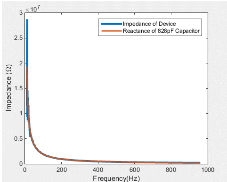
Figure 11. Impedance of PEH and reactance of 828pF capacitor
