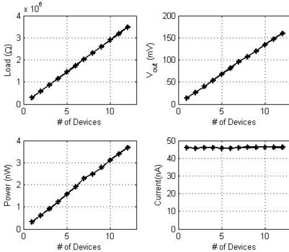
Figure 24. Matched load, output voltage, power, and current of devices connected in series
