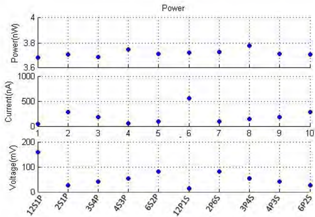
Figure 25. Power, current, and voltage calculations of 12 devices connected in series and in parallel
