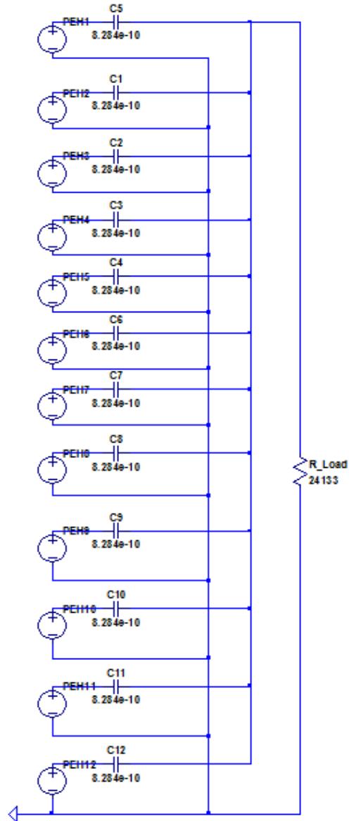
Figure 21. Twelve PEHs connected in parallel
