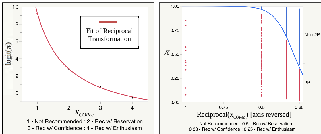
Figure 5. Log-Odds (left) and Logistic Fit (right) of 2P Staff Sergeants by Commander’s Recommendation. The plot of log-odds reveals a reciprocal relationship where a lower Zone C Commander’s Recommendation is correlated to a higher 2P likelihood (Chi-Squared = 517; p-value < 0.01). The x-axis of the logistic fit has been reversed to keep lower recommendations on the left hand side of the axis.
