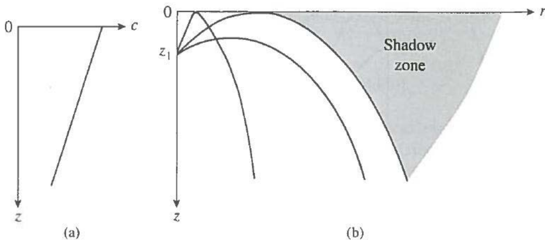
Figure 6. Diagram of an acoustic ray trace
