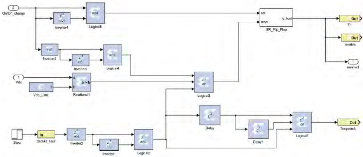
Figure 4.1. The original fault management circuit design in Simulink.
