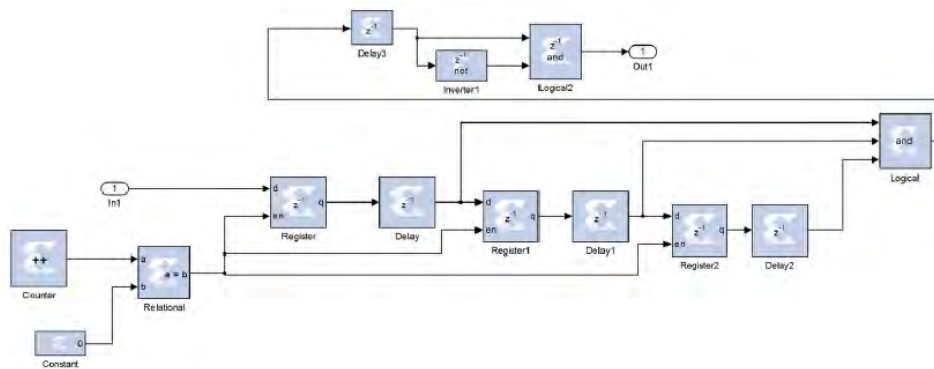
Figure 4.5. The first new fault detection circuit to overcome the EMI issues.
