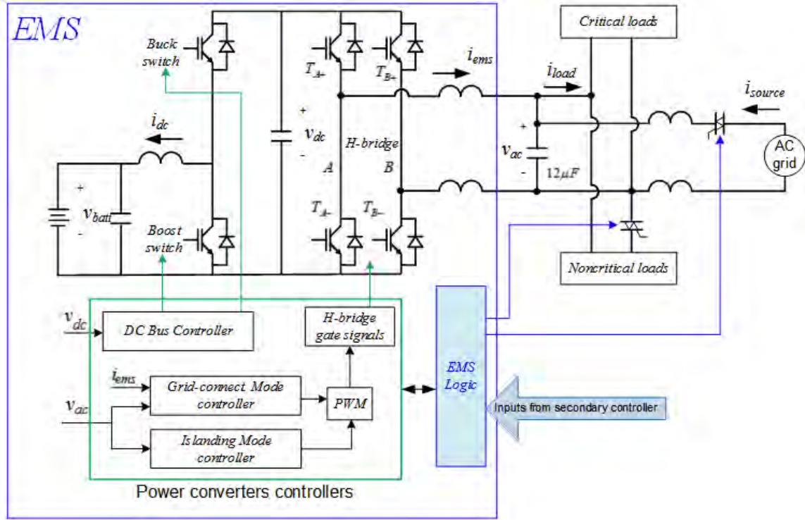
Figure 2.1. The basic topology of a power electronics-based EMS, from [13].
