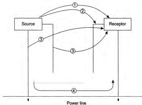
Figure 5. Mechanisms of Electromagnetic Interference (from Kodali 2001)
