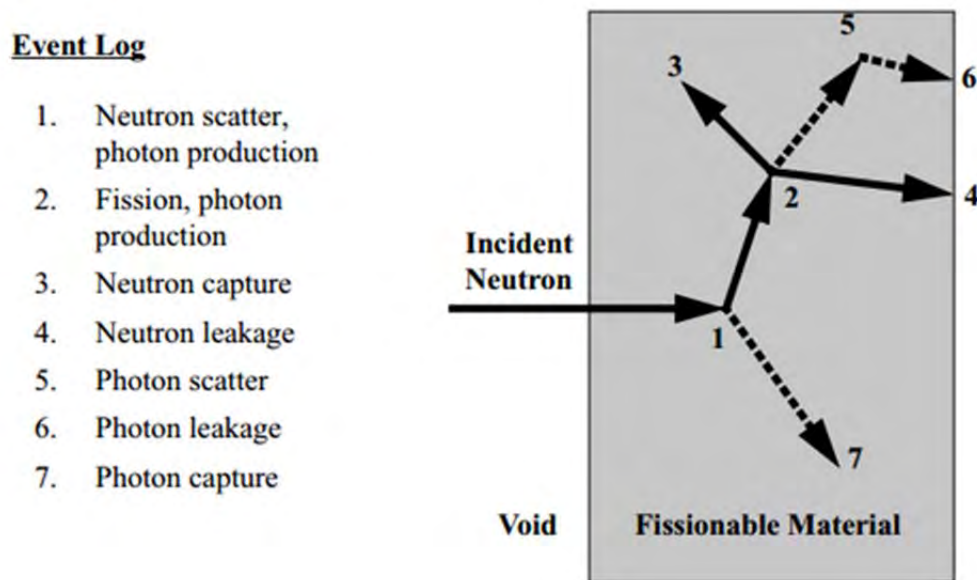
Figure 8. MCNP history of neutron incident on fissionable material with numbered events, from [7].
