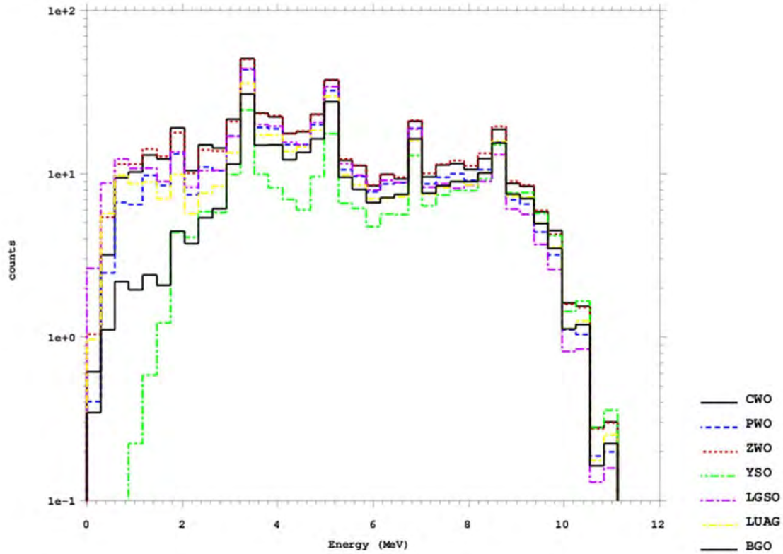
Figure 16. Inelastic scatter of each crystal against neutron energy. Lower black line is BGO.
