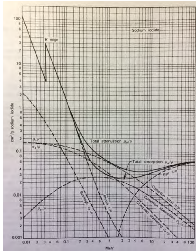
Figure 1. Cross sections for gamma interactions with sodium iodide vs. incident gamma energy, from [9].
