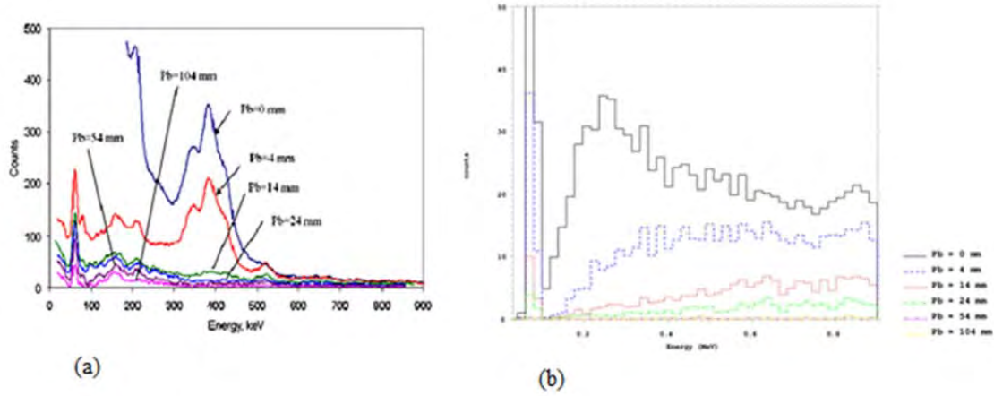
Figure 20. (a) Experimental measurements of CWO with low energy PuBe gamma spectra with different Pb shield thicknesses. (b) MCNP energy deposition calculations in CWO with flat distribution of gamma in equivalent energy range.
