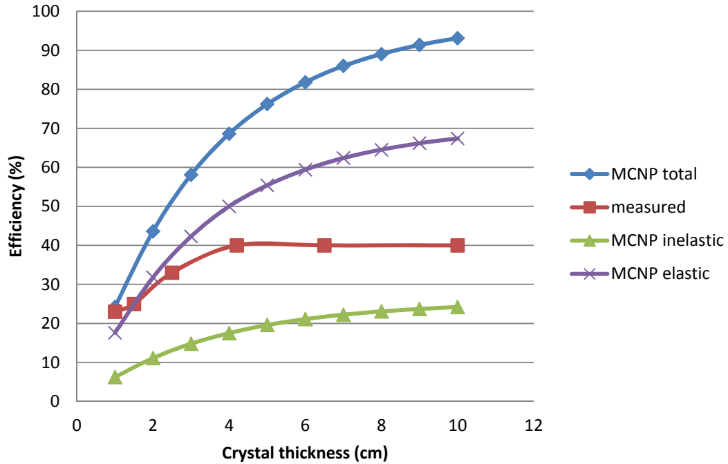
Figure 28. Measured detection efficiency with calculated efficiency of total interactions, elastic scattering, and inelastic scattering in CWO with increasing crystal thickness.
