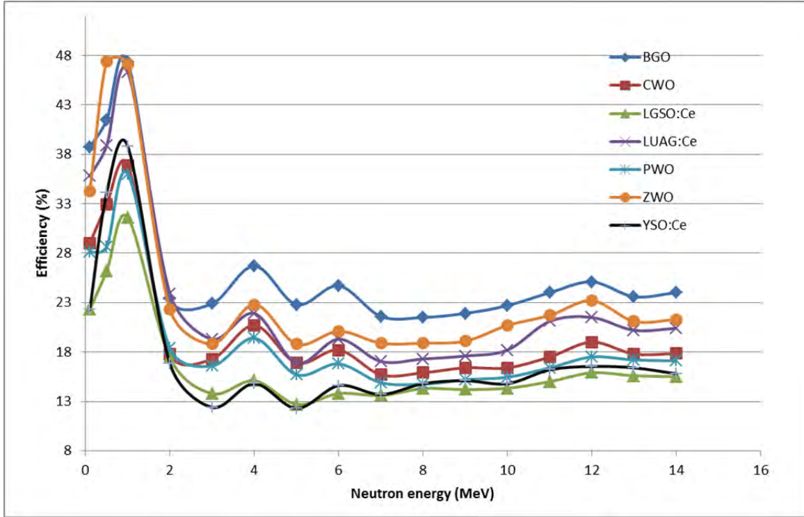
Figure 27. Response function of basic detector configuration exposed to PuBe neutron source for each crystal modeled with MCNP.
