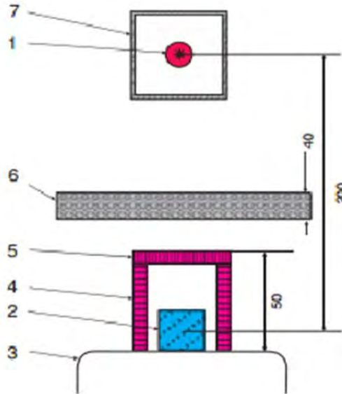
Figure 19. Basic experimental set up for crystal experiments in NASU.
