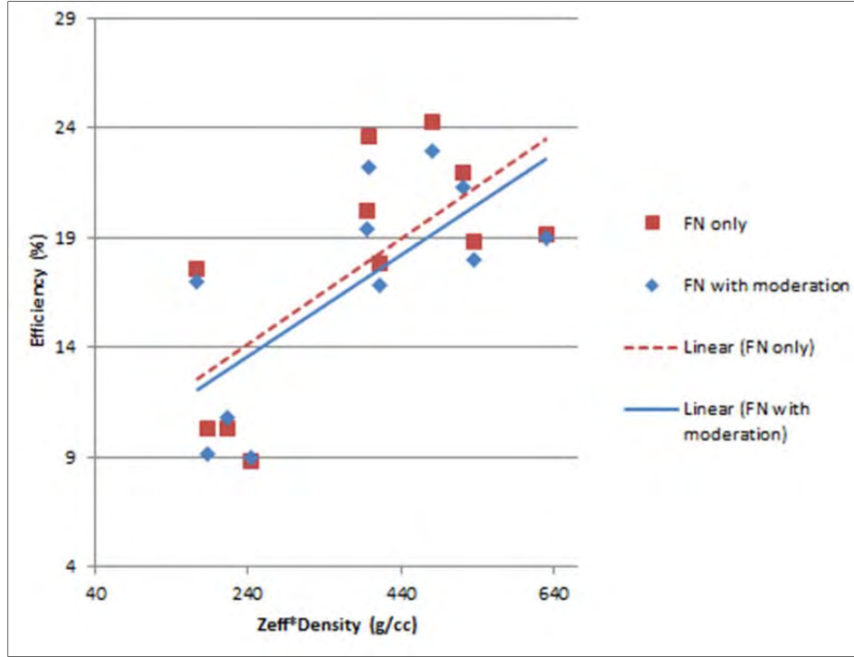
Figure 26. Calculated efficiency vs. effective atomic number times density in g/cc.
