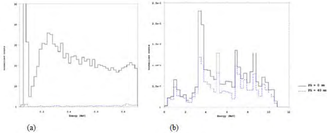
Figure 21. (a) CWO energy deposition from gamma radiation in 0-900 keV with Pb shield thickness of 0 mm (black) and 40 mm (blue). (b) CWO energy deposition from PuBe neutron source in energy range from 0–12 MeV with Pb shields of 0 mm (black) and 40 mm (blue).
