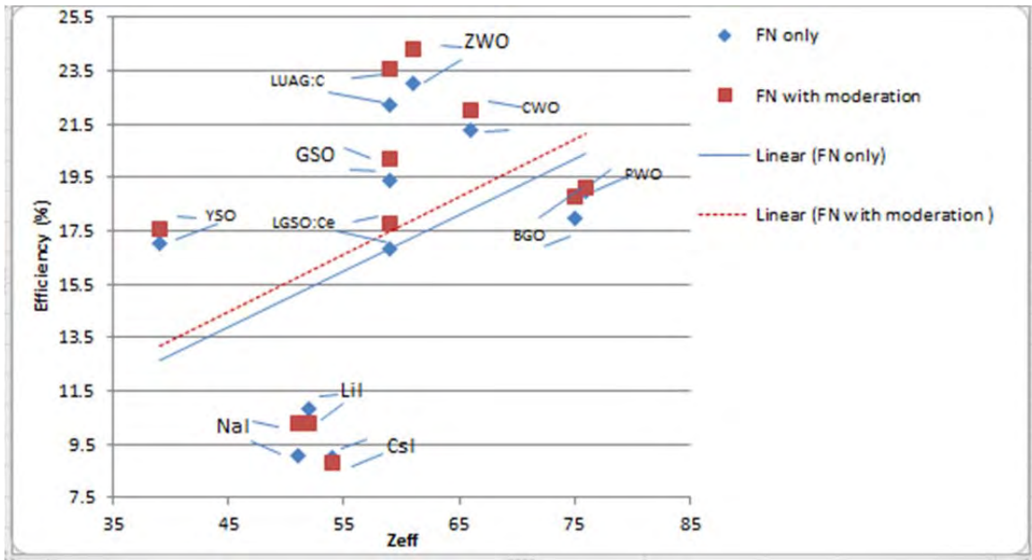
Figure 25. MCNP approximation of detection efficiency for several inorganic scintillator crystals with (red) and without (blue) moderation.
