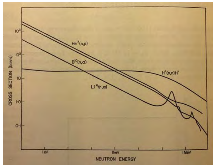
Figure 3. Log-log plot of neutron absorption or scattering cross sections for four neutron detection process vs. neutron energy, from [9].
