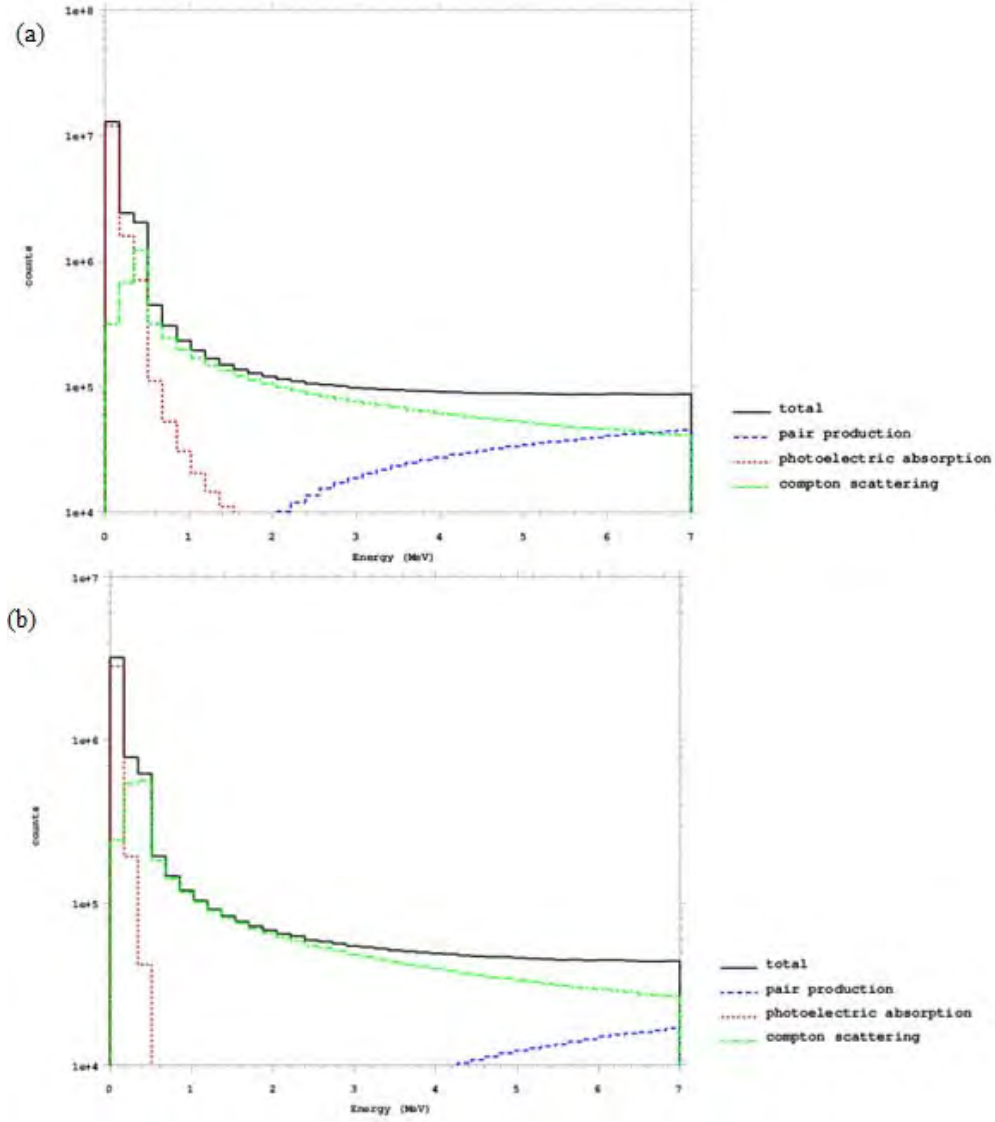
Figure 12. (a) ZWO reactions from incident gamma spectrum. (b) YSO reactions from incident gamma spectrum.
