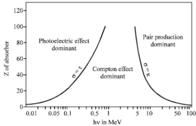
Figure 2. Behavior of gamma interaction with matter with respect to Z number and incident gamma energy. Solid lines mark equal probability of processes, from [10].
