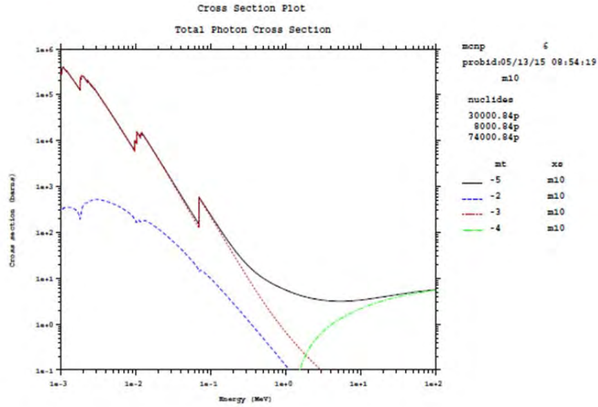
Figure 10. MCNP Cross Section plot of photon cross sections for ZWO: -5 is total cross section, -2 is Compton scatter, -3 is photoelectric abs., and -4 is pair production.
