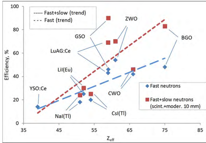
Figure 24. Detection efficiency of fast and thermal neutron from fluxes from PuBe source measured by inelastic scattering at ISM, Ukraine, from [14].
