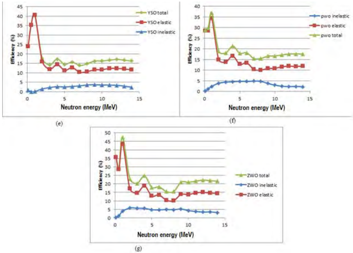
Figure 18. Response curves for (e) YSO, (f) PWO, and (g) ZWO based on the upper limit of detection efficiency discussed above.
