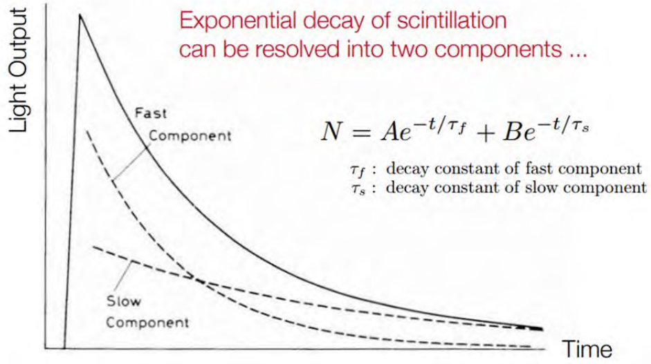
Figure 7. The total relaxation of luminescent crystal shown as sum of slow and fast exponential decay, from [11].
