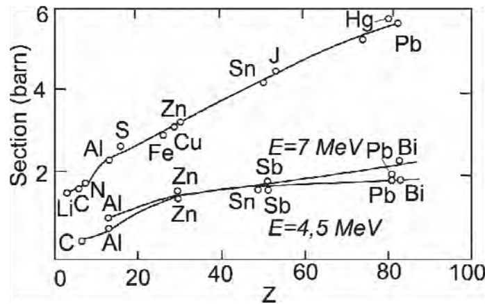
Figure 4. Cross section of total interactions (top line) and inelastic scattering (bottom 2 lines) of various elements vs. atomic number, at neutron energy of 7, 5, and 4 MeV, from [6].
