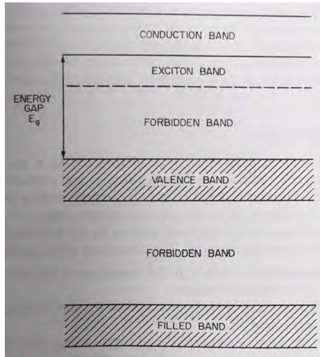
Figure 5. Energy band structure of ideal insulating crystal, from [9].
