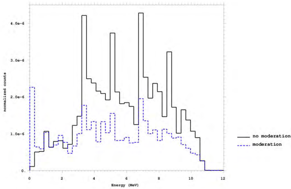
Figure 23. Energy deposition in CWO by PuBe neutrons with (blue) and without (black) moderation.
