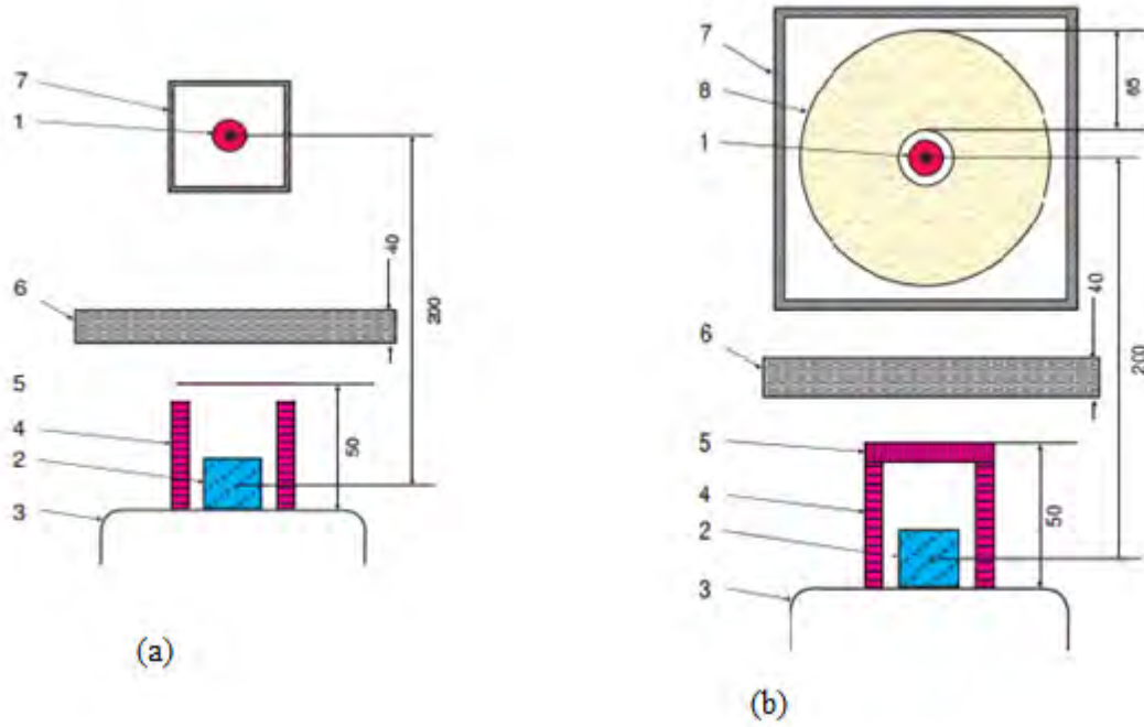
Figure 22. (a) experimental setup without moderation. (b) experimental setup with 8-polyethylene moderator around source and 5-gadolinium oxide lid.
