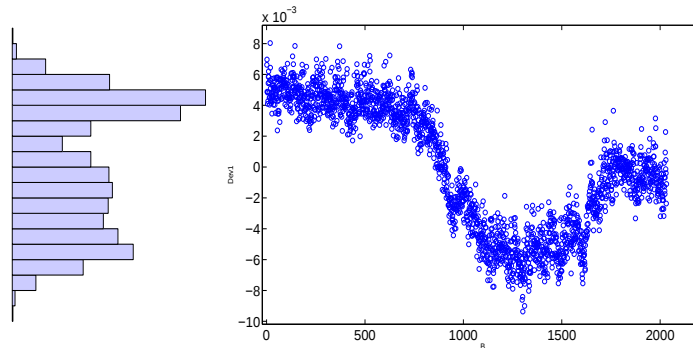
Figure 26. Run 1, histogram showing peak standard deviation \sim 0.004 W
