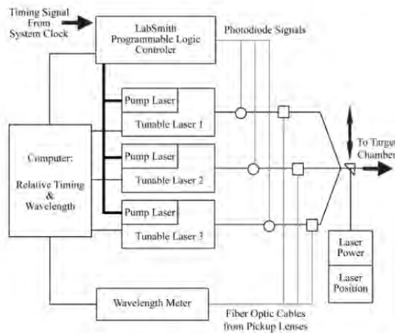
Figure 2. Current RIMS pump and ionization laser setup, from [2]
