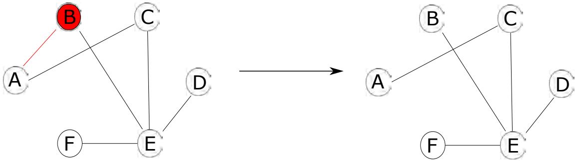
Figure 2.9: A reduction by the DRVE method. First, a random vertex from the node-set is selected, in this case, B . Next, the edge (B, A) is randomly chosen from the edges incident to B , and removed from the graph. A check is done for graph connectedness, and only the largest connected component is retained. In this example, the graph remains connected after edge deletion.
