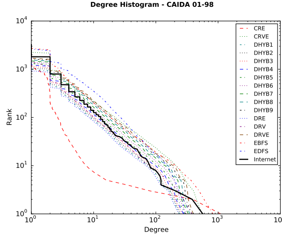
Figure 5.21: Degree histogram of reduction methods versus 1 January 1998 Internet graph – CAIDA 2001–1998
