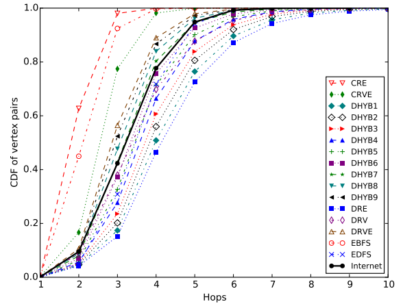
Figure 5.10: Hop plot of reduction methods versus 24 January 1998 Internet graph – RouteViews 2001–1998
