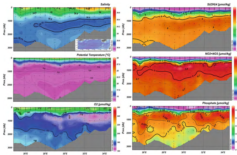
Figure 16. Vertical Sections of Dissolved Oxygen and Nutrients along West-East Cross Section of the Levantine Basin
