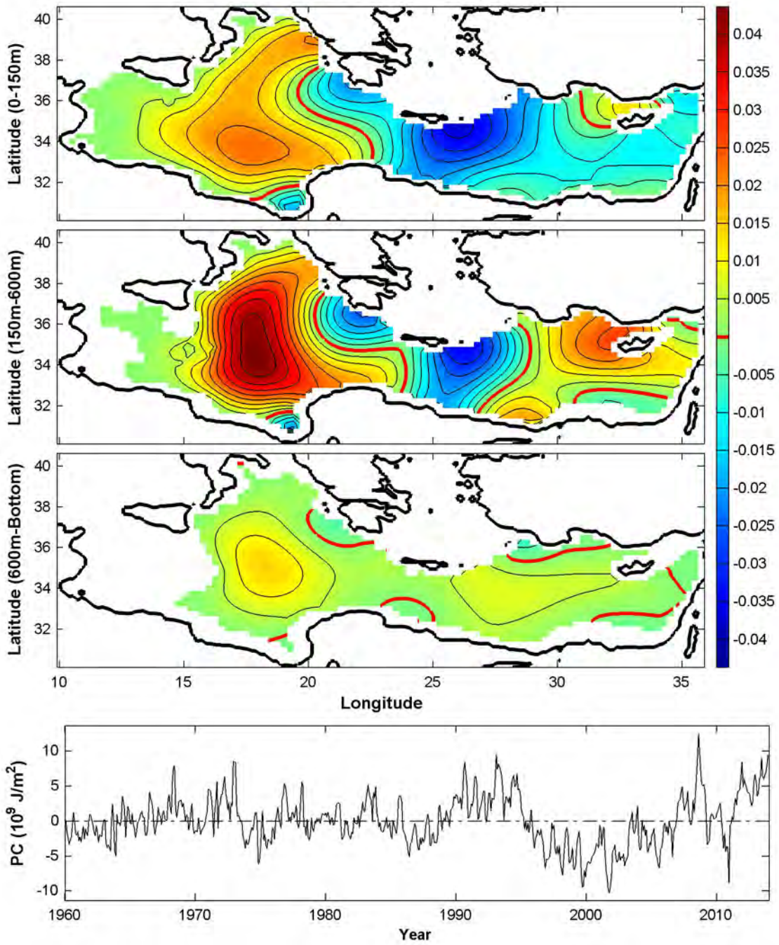
EOF of Heat Content (Mode: 3) 6.02%
