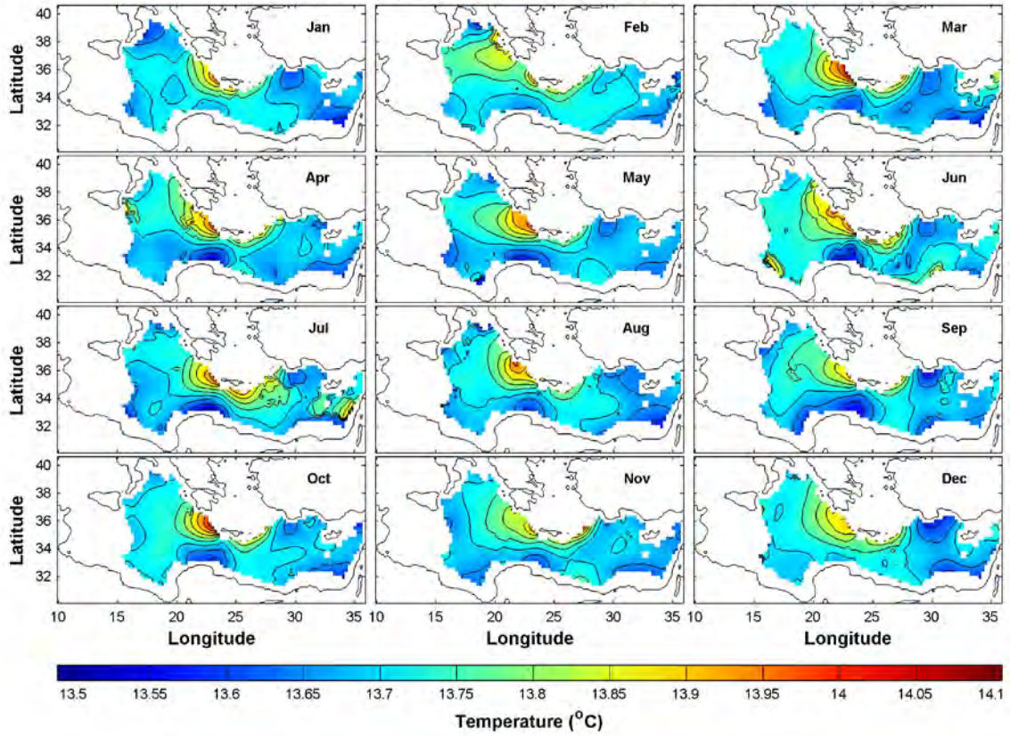
Monthly Mean Temperature at Depth: 1000m
