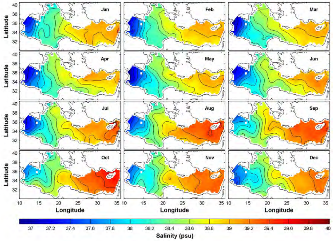
Monthly Mean Salinity at Depth: 10m
