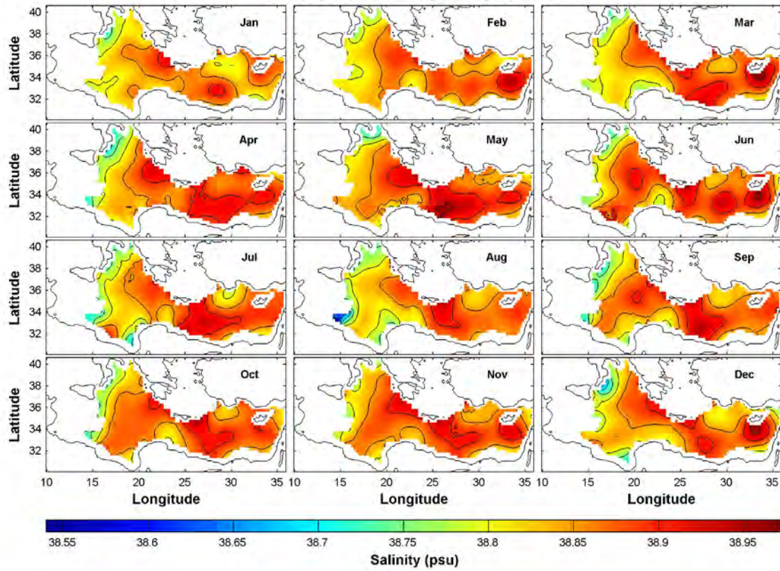
Monthly Mean Salinity at Depth: 400m
