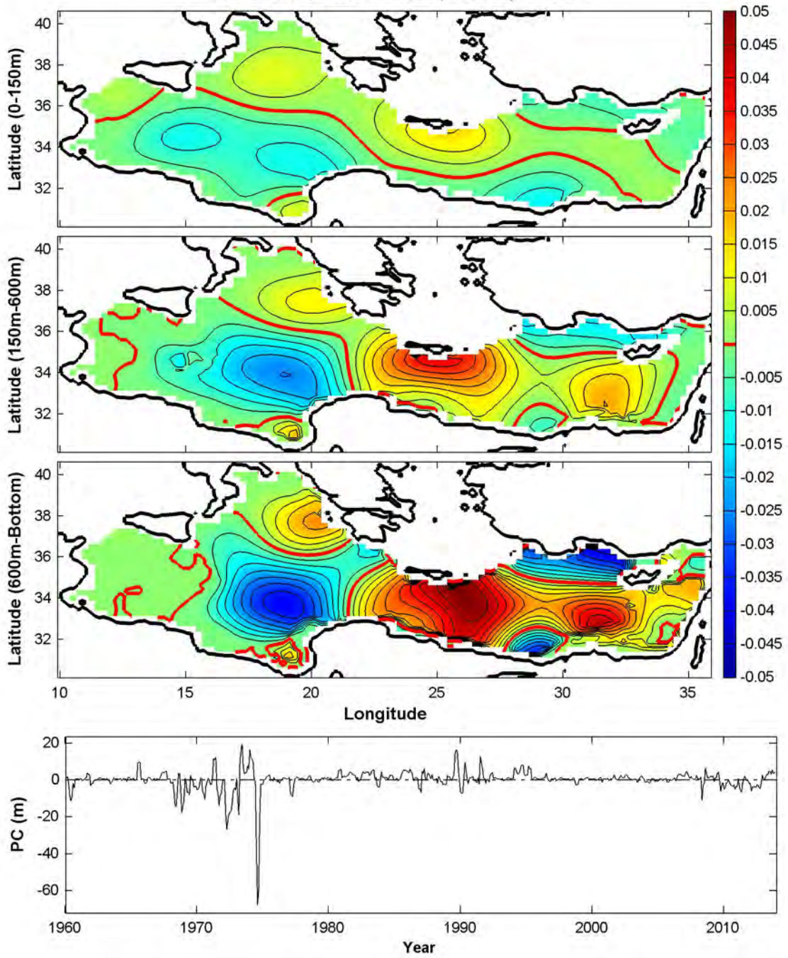
EOF of Freshwater Content (Mode: 3) 8.47%
