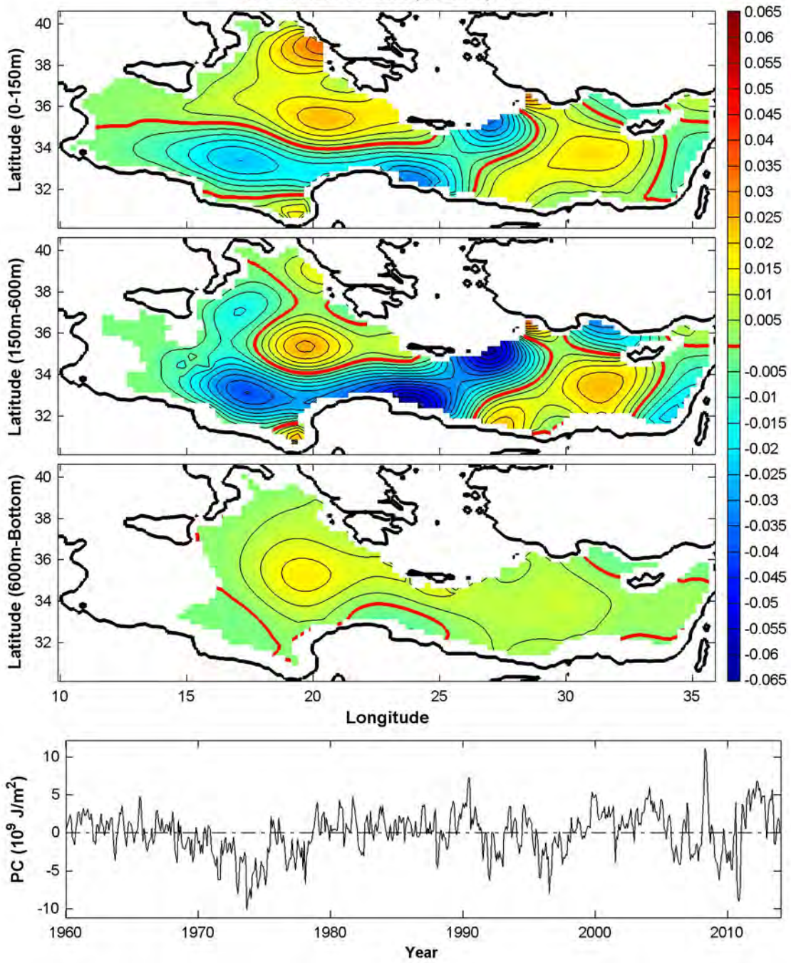
EOF of Heat Content (Mode: 5) 4.27%
