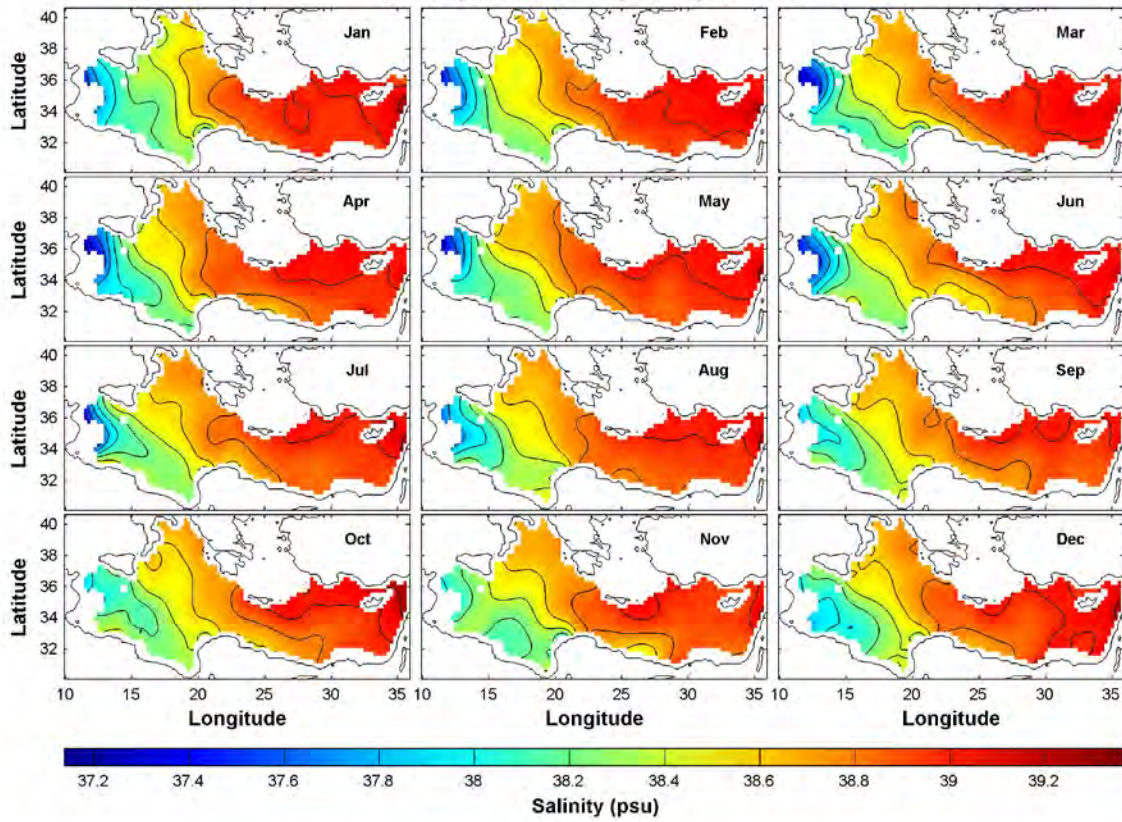
Monthly Mean Salinity at Depth: 100m
