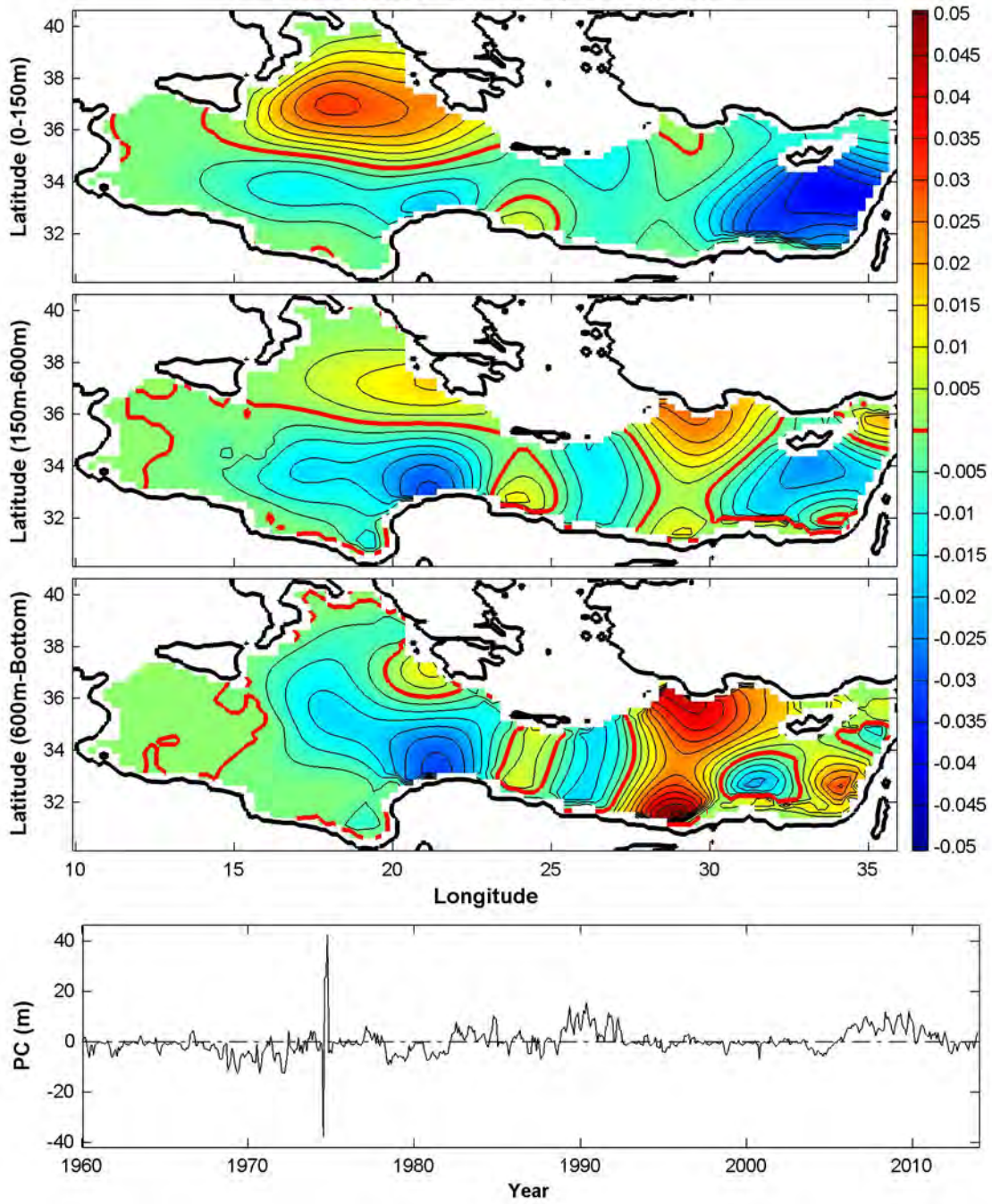
EOF of Freshwater Content (Mode: 4) 6.3%
