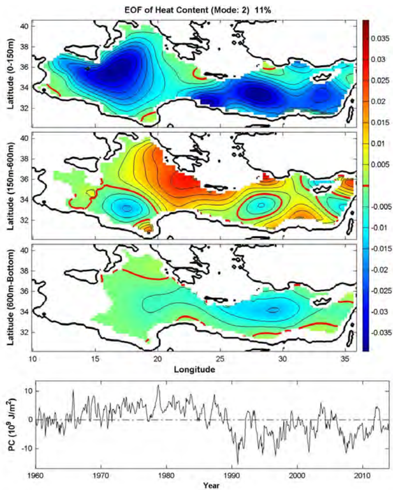
Figure 51. EOF Mode-2 and PC-2 of Surface Layer (0-150m), Intermediate Layer (150-600m) and Deep Layer (600-bottom) Heat Content ( J/m^2 )
