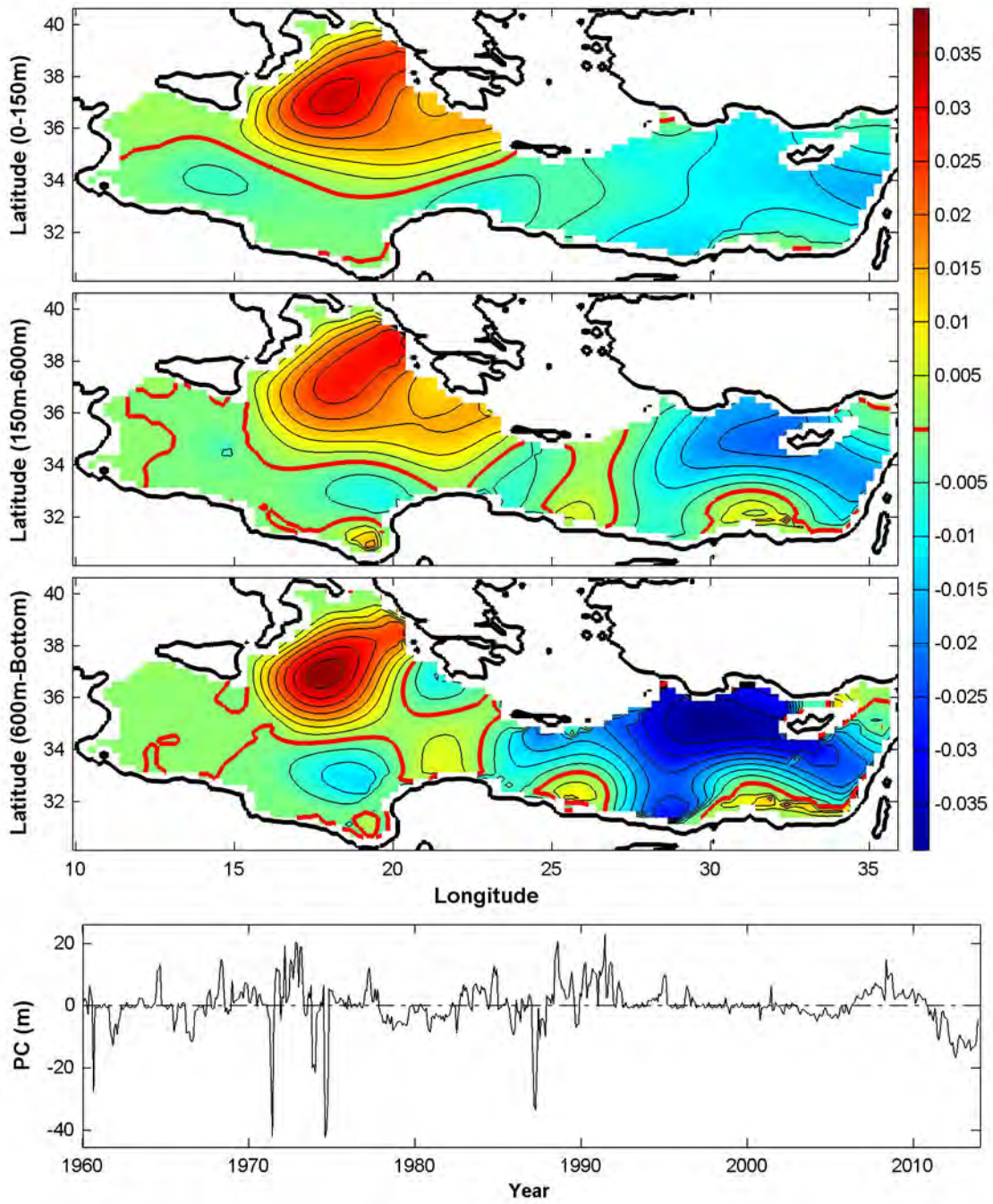
EOF of Freshwater Content (Mode: 2) 11.9%
