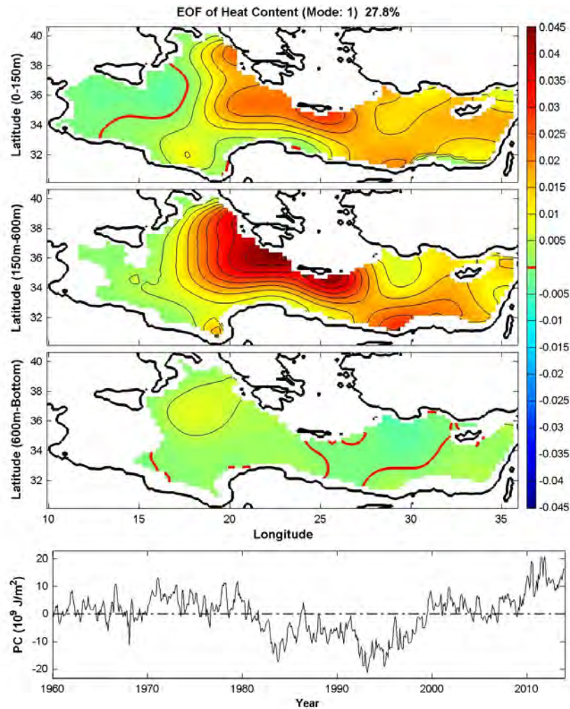
Figure 50. EOF Mode-1 and PC-1 of Surface Layer (0-150m), Intermediate Layer (150-600m) and Deep Layer (600-bottom) Heat Content ( J/m^2 )
