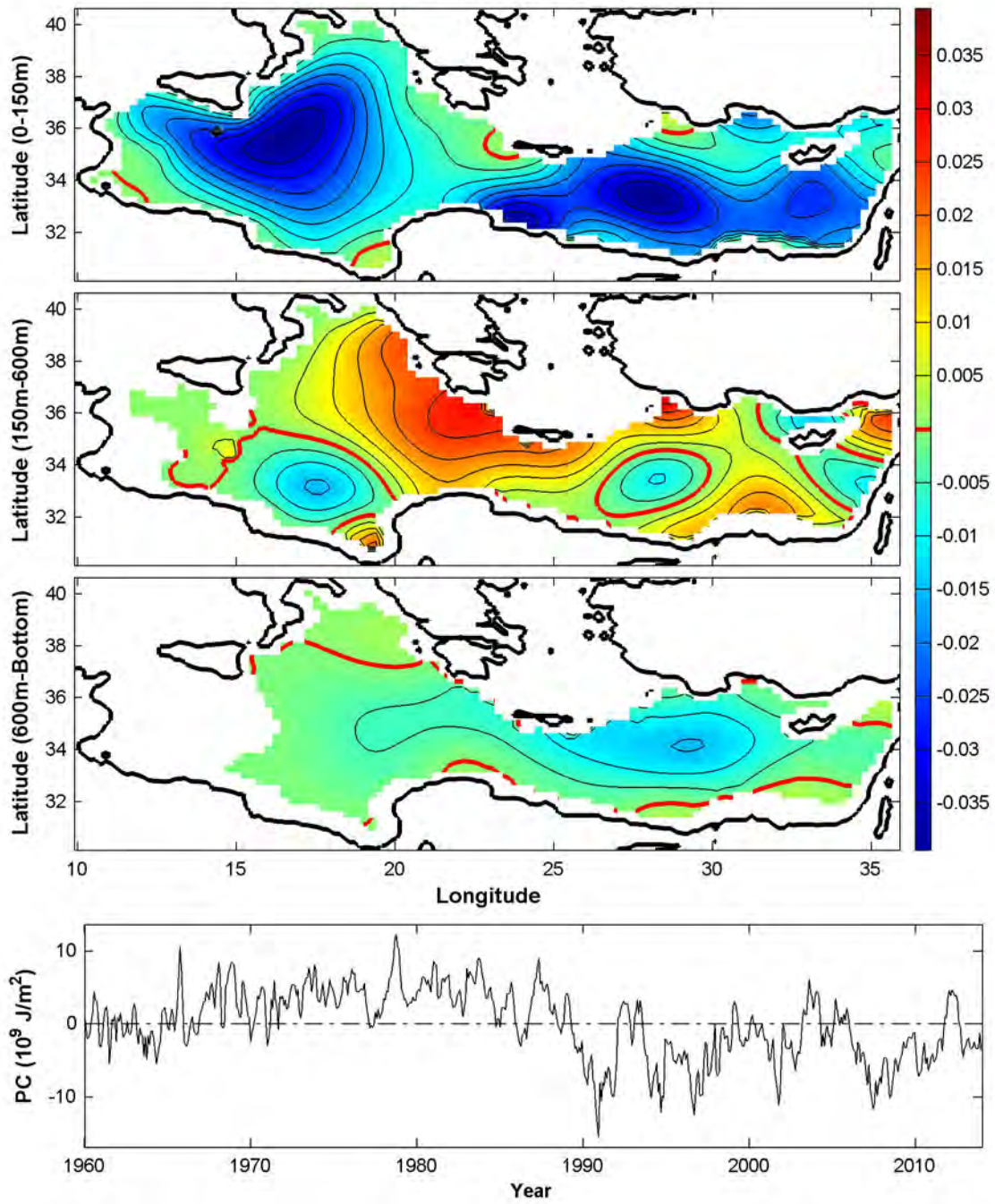
EOF of Heat Content (Mode: 2) 11%
