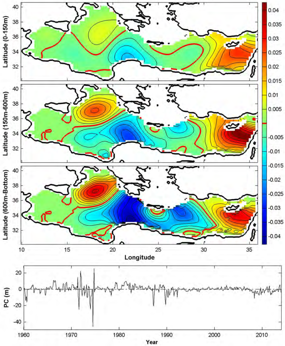
EOF of Freshwater Content (Mode: 5) 5.65%
