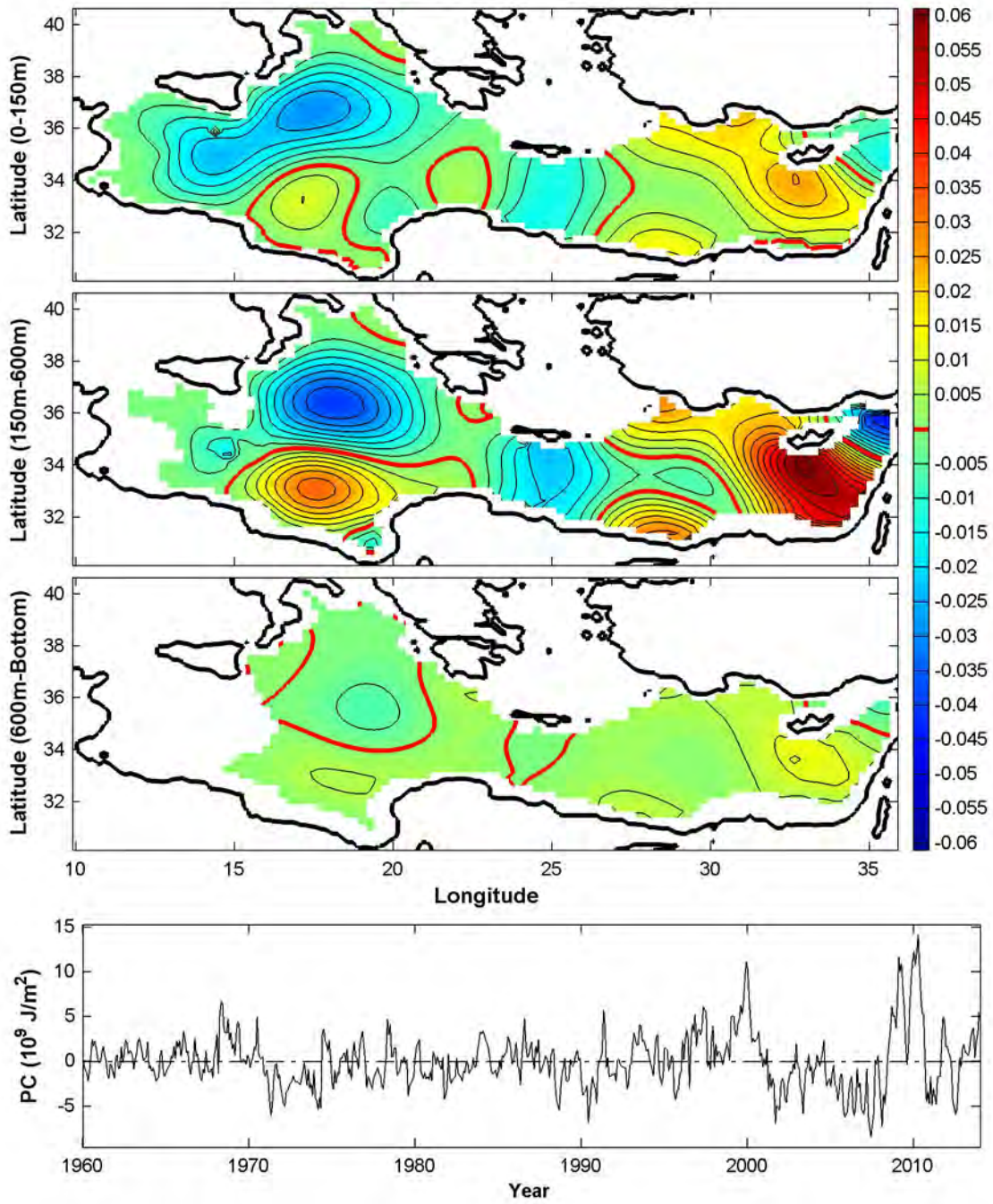
EOF of Heat Content (Mode: 4) 4.65%
