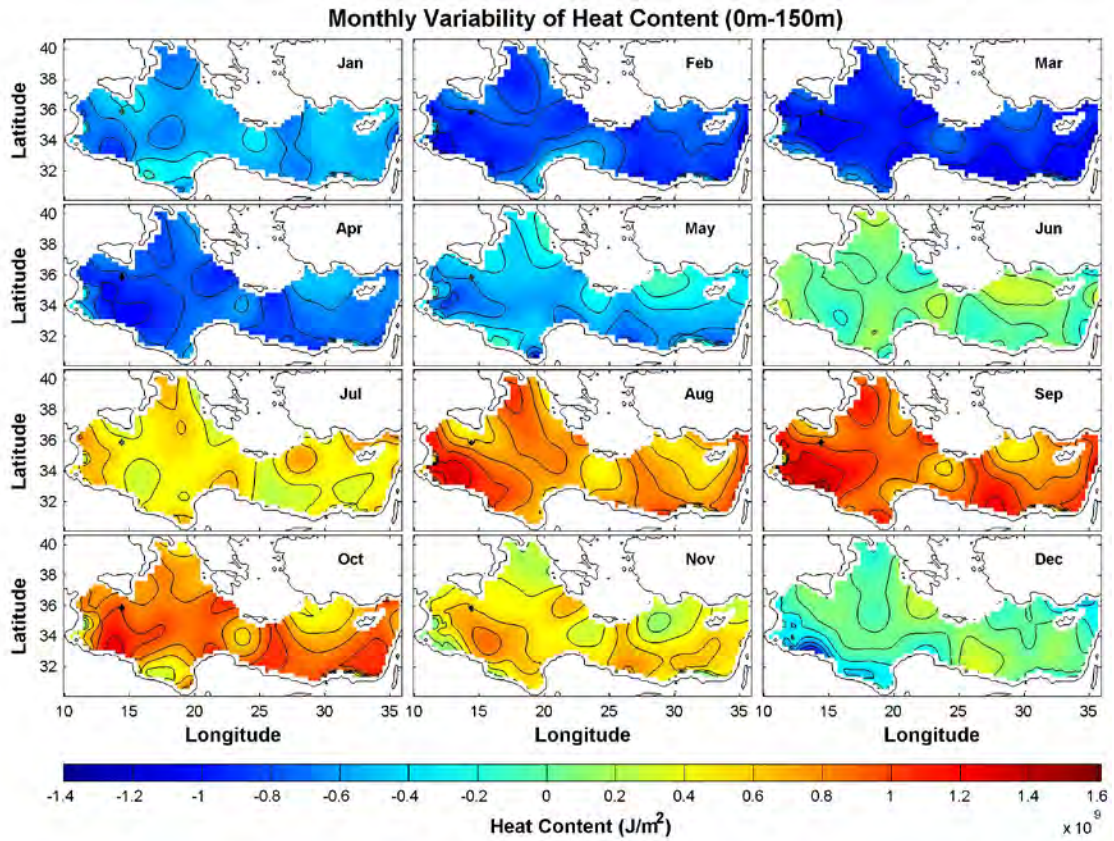
Figure 44. Monthly Variability of Heat Content ( J/m^2 ) at the Surface Layer
