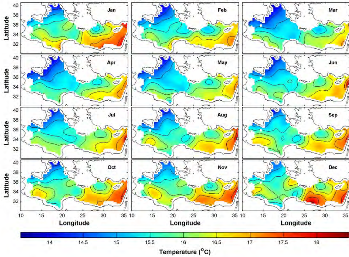
Monthly Mean Temperature at Depth: 100m
