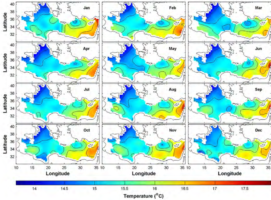
Monthly Mean Temperature at Depth: 150m
