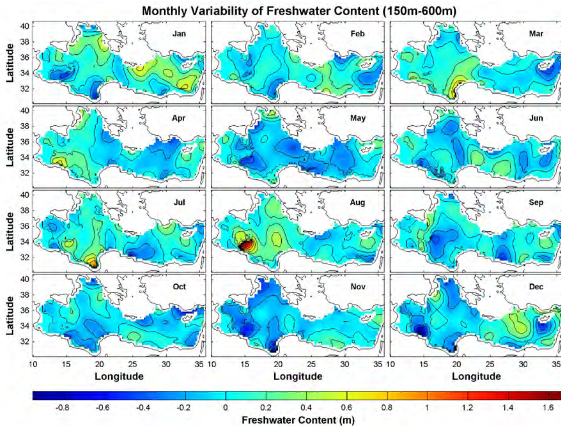
Figure 48. Monthly Variability of Freshwater Content (m) at the Intermediate Layer
