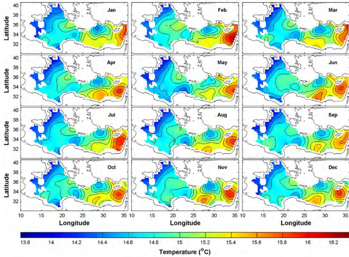
Monthly Mean Temperature at Depth: 250m
