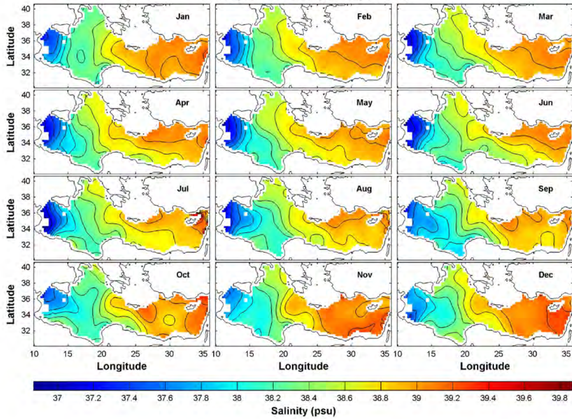
Monthly Mean Salinity at Depth: 50m
