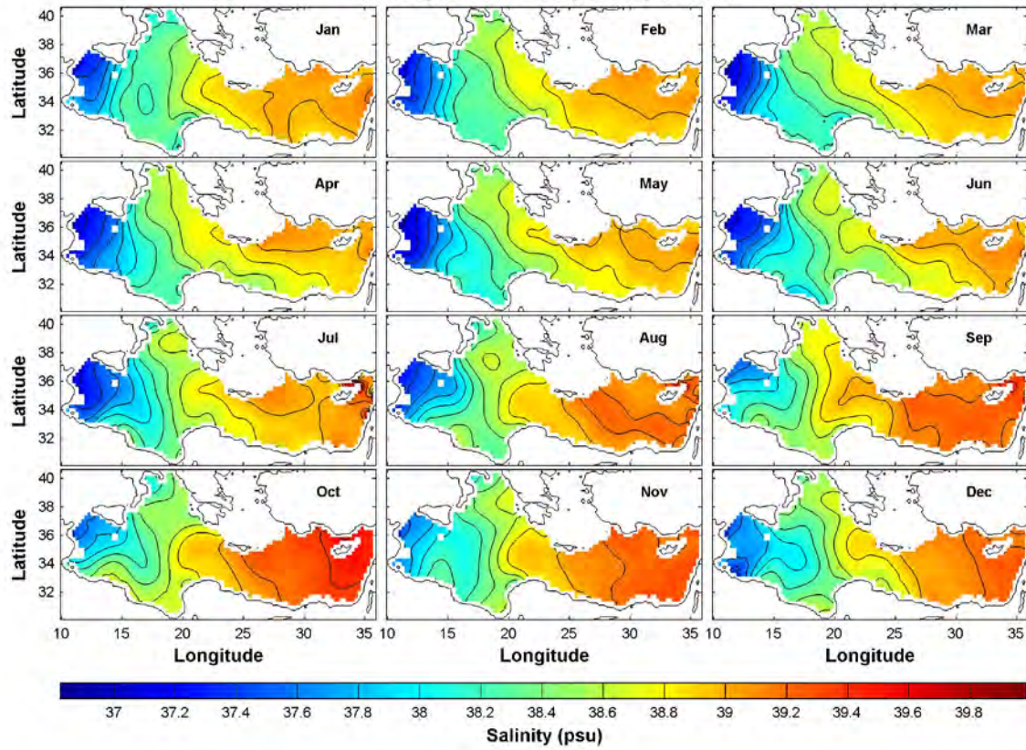
Monthly Mean Salinity at Depth: 20m
