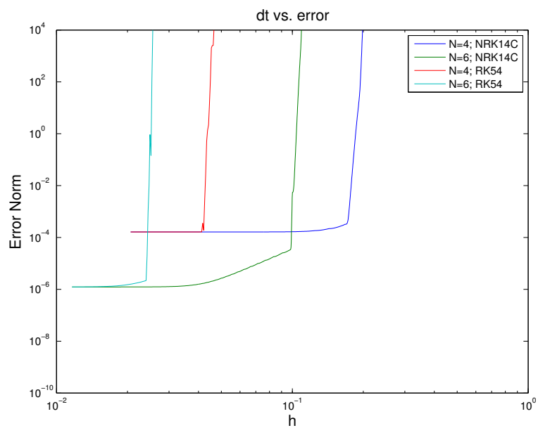
Figure 3.8: Shows error versus h with N = 4 and 6 polynomial order using the mesh from Figure 3.7(b).
