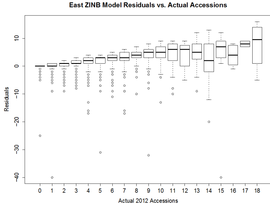
Figure 36. Plot of the residuals (actual accessions minus predicted accessions) versus the actual accessions for the east ZINB model, indicating a slight positive trend diverging from 0 residuals up to 12 accessions where the mean begins to re-converge with 0 residuals and eventually plateaus.
