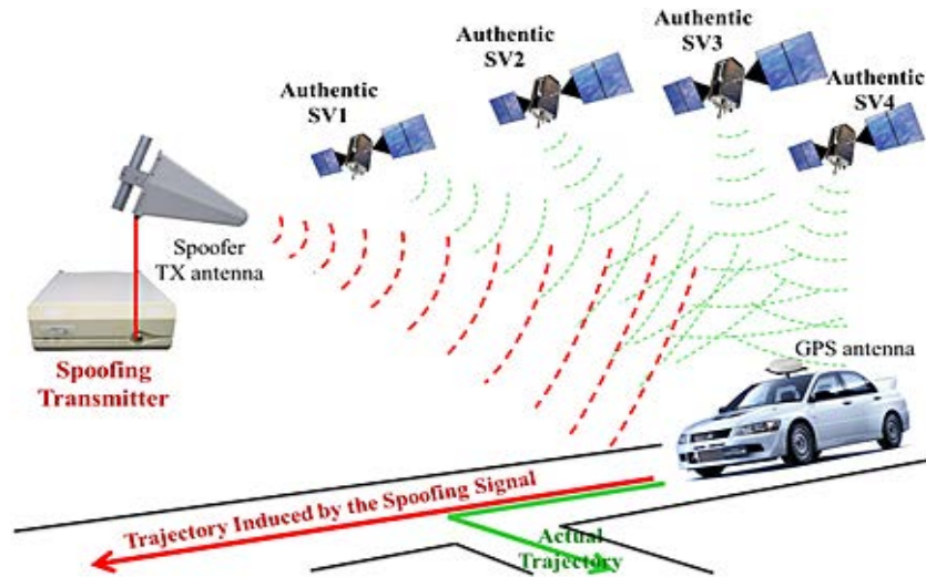
Figure 17. Effects of Spoofing on Navigation Systems, from [26].
