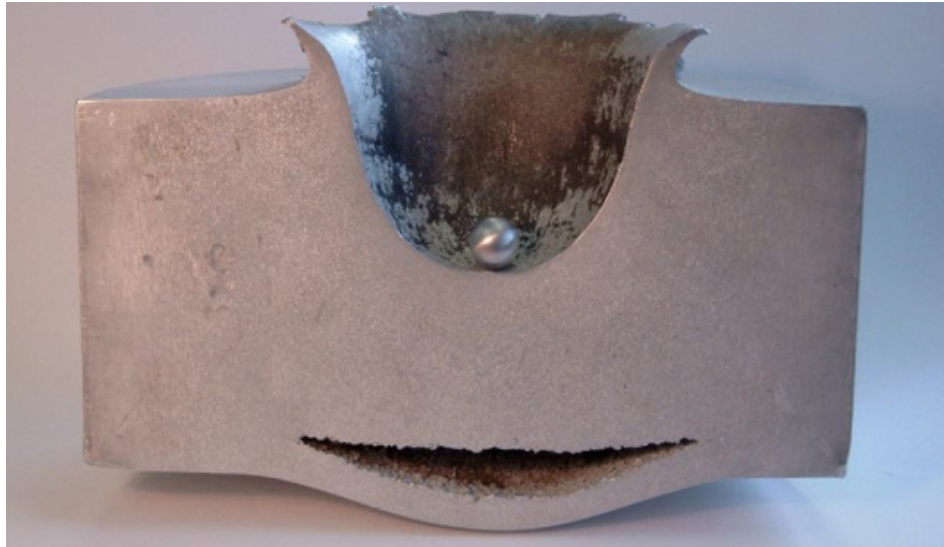
Figure 9. Results of a Half-Inch-Wide Impactor Striking a 7-inch-thick Aluminum Block at 15,200 mph (6.8 km/s), from [23].
