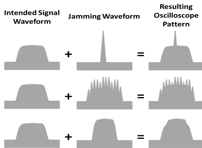
Figure 23. Example of Oscilloscope Readout with Interference, after [24].
