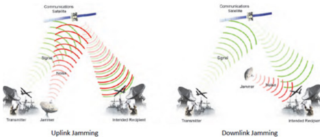
Figure 16. Examples of Uplink and Downlink Jamming, from [25].
