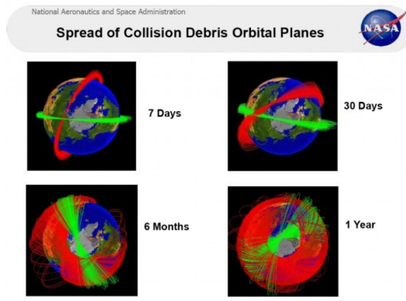
Figure 8. Debris Spread from the Iridium-Cosmos Collision over Time, from [23].
