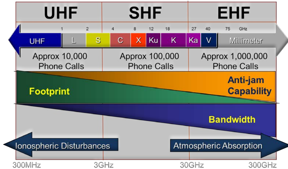
Figure 18. Satellite Communication Frequency Bands, from [26].
