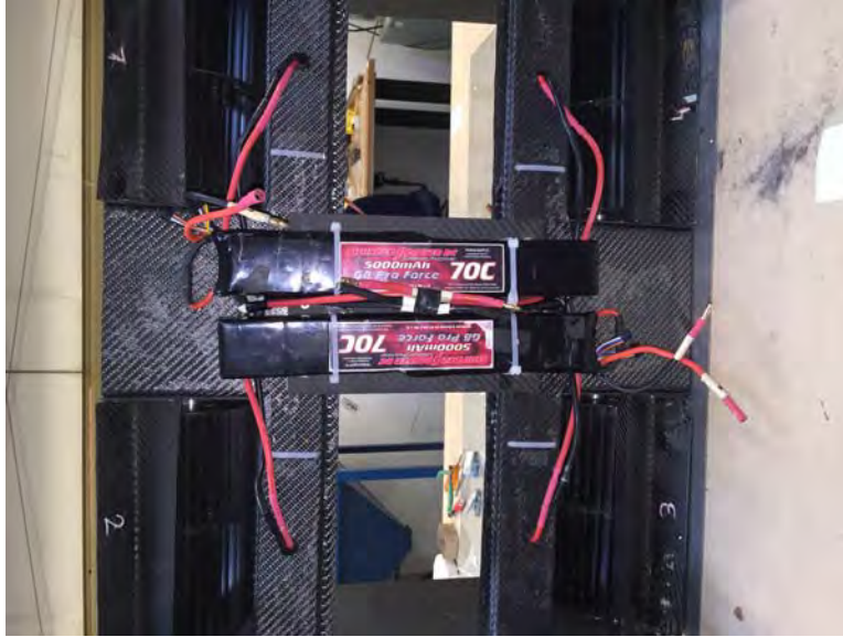
Figure 75. LiPo batteries and parallel battery connector cable.
