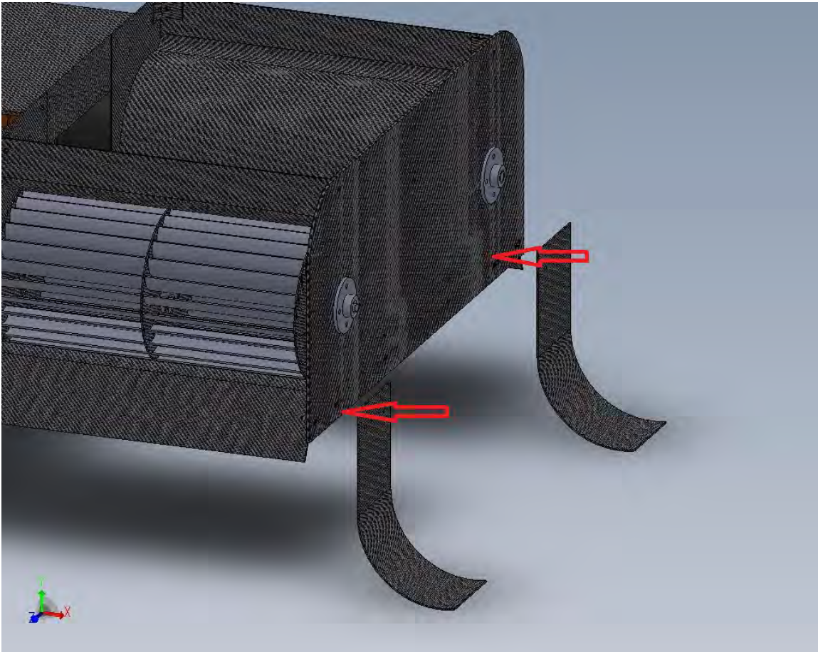
Figure 71. Landing gear.
