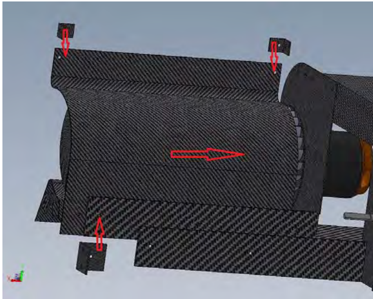
Figure 65. Intake housing to airframe foundation.
