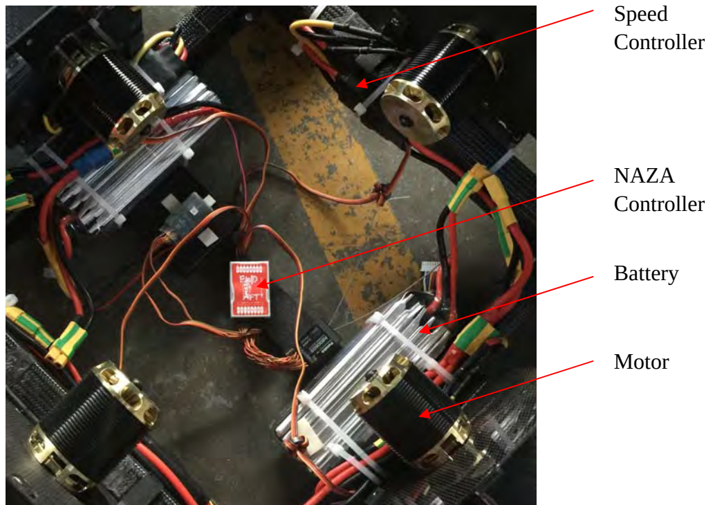
Figure 31. Third-generation wiring harness layout.
