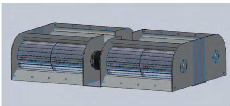
Figure 12. SolidWorks design, Generation 1. From [2].
