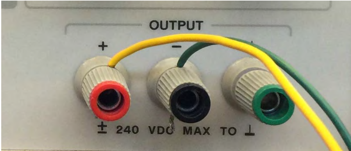
Figure 84. Speed control console to DC power supply connection.
