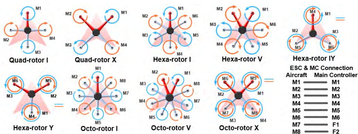
Figure 34. NAZA-M motor configuration options, from [22]
