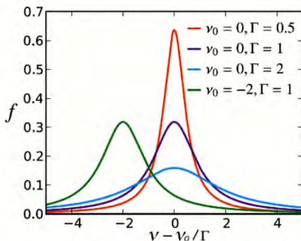
Figure 4. Resonant frequency and the damping dependence of the spectral line width. From [16].
