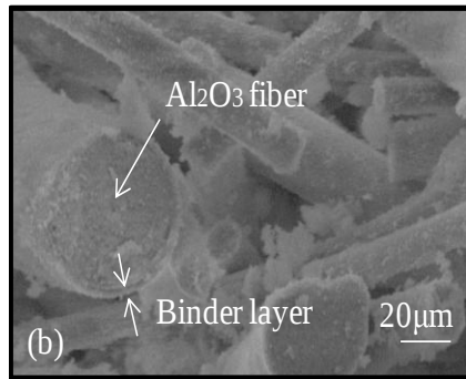
Fig.1. SEM images of Al 2 O 3 fiber (a), fiber and SiO 2 binder inside preform
