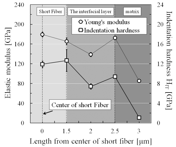
Fig.6. Young' modulus and indentation hardness from each position.
