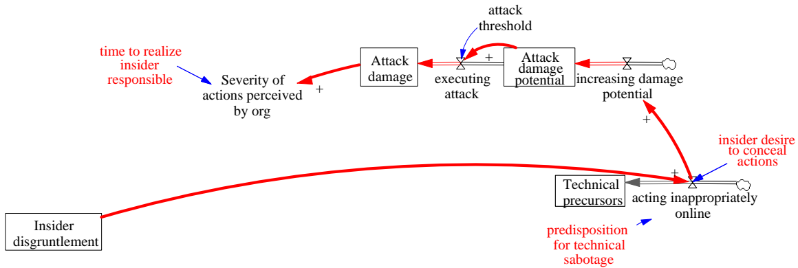
Figure 9: Attack Escalation
