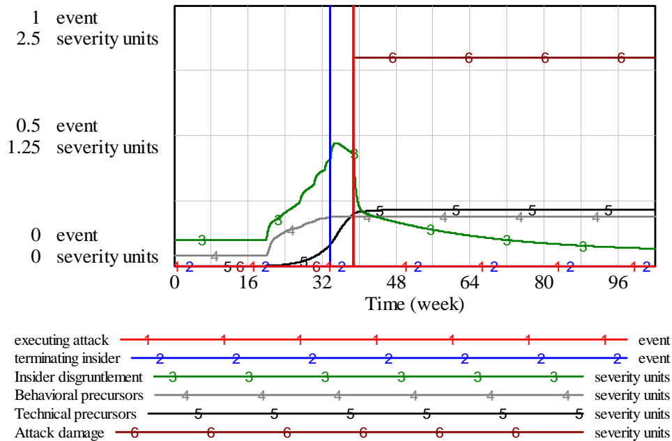
Figure 10: Attack Simulation
