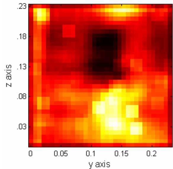
Figure 4. Measurement results show decrease in longitudinal energy caused by 2.5×5×7 cm steel inhomogeneity located at x = 11.75 (2 cm deep), y = 0.12 , z = 0.15 .
