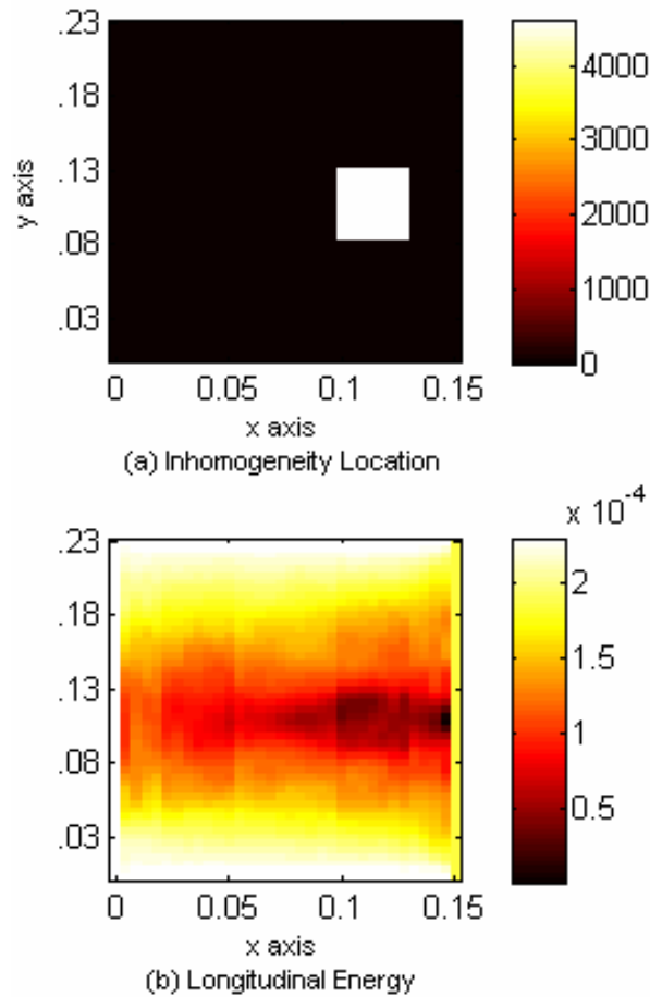
Figure 3. FDTD simulation results: (a) inhomogeneous region sound speed depicts location of 2.5×5×7 cm steel inhomogeneity; and (b) simulation results show weak longitudinal energy at L_a = 0.15 surface due to inhomogeneity.
