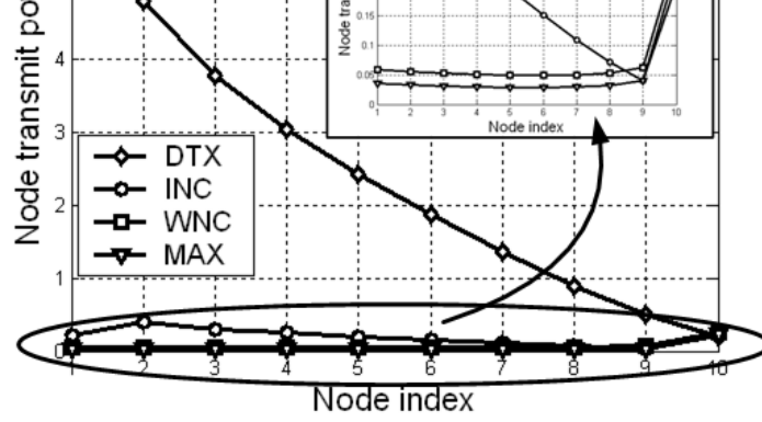
Figure 3.6: Distribution of transmit power in DTX, INC, MAX, and WNC ( \rho = 0.5 ) for a 10-unit network.
