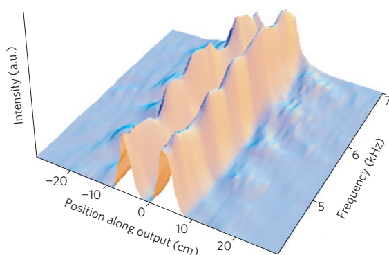
Figure 4 | The broadband performance of the acoustic hyperlens.
