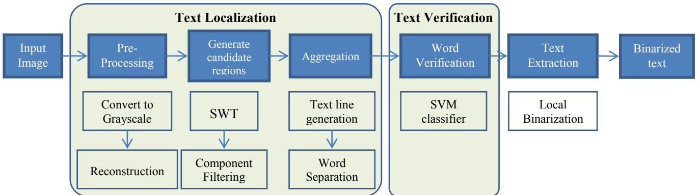
Fig. 1. The flowchart of the proposed text detection and extraction method
