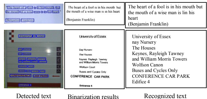
Fig. 10. Binarization results and recognition results by the proposed methods
