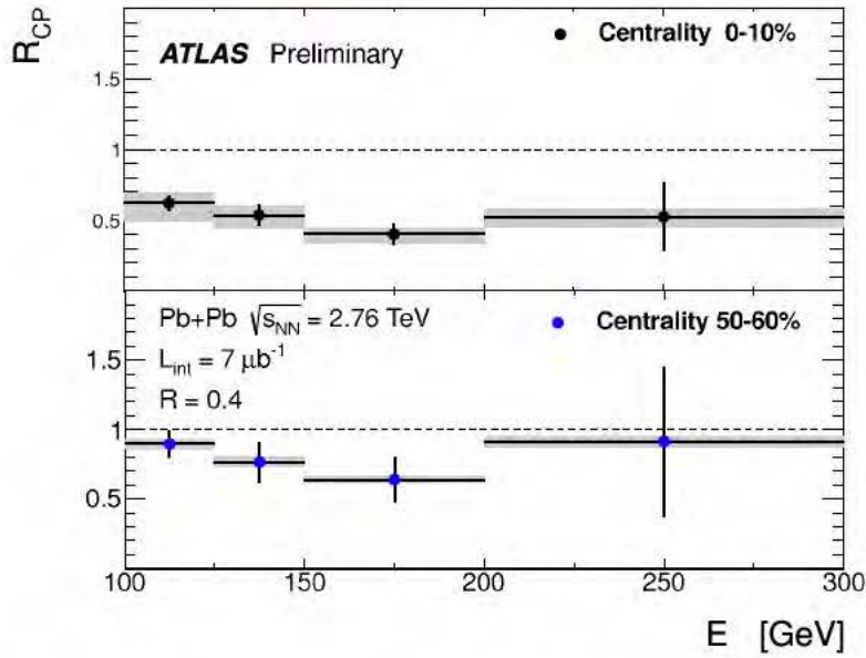
Figure 19. The jet central-to-peripheral ratio R_{CP} for different centralities in Pb–Pb collisions at the LHC, measured by the ATLAS collaboration [273]. The plots show the ratio of the jet yield in central 0–10% and semi-peripheral 50–60% events relative to the yield in very peripheral collisions as a function of the transverse energy E_T of the jet.
