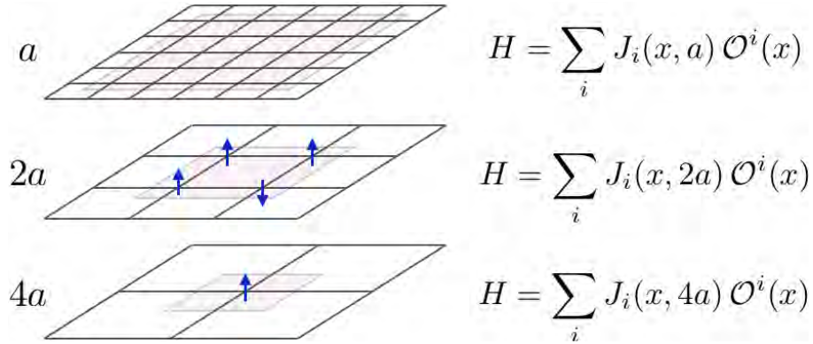
Figure 22. Coarse-graining spins on a lattice à la Kadanoff and Wilson. At each step we coarse-grain by replacing the degrees of freedom on a block of sites by an average value on a single site, rescaling the lattice spacing a and tuning the couplings J_i(x, a) in the Hamiltonian H so that the physics of the ground state and low-lying excitations remain invariant under the scaling operation.
