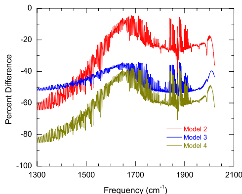
Figure 5. Percent difference ( =[(\text{model } x - \text{model } 1)/\text{model } 1] * 100 , x = 2, 3, and 4 ) in the calculated radiances using different models as a function of frequency.
