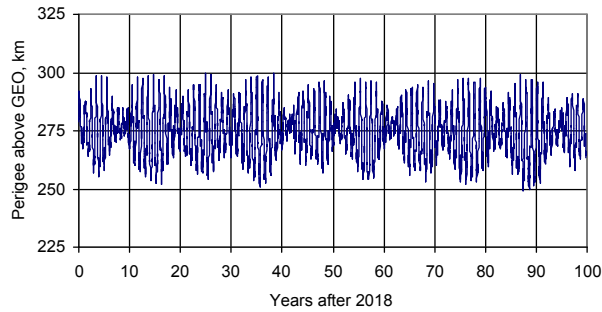
Figure B.2. 100-year perigee history (Sun-pointing).
