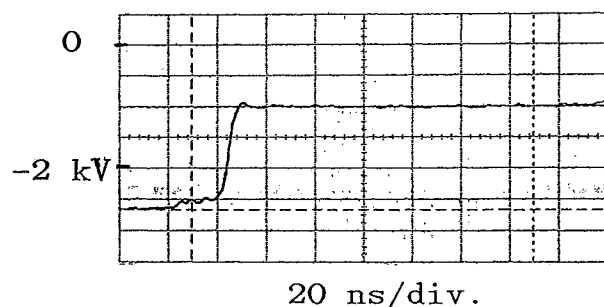
Figure 3. The voltage (0.5 kV/div) across an ITC-treated GaAs switch as function of time (20 ns/div). The switch was triggered by 14 \mu\text{J} of 1060 nm light, that causes the first slight decrease in voltage (from 2.67 kV to 2.5 kV). The current at this point is 2.5 A. After a delay of about 20 ns, the switch locks-on. The lock-on voltage is 1.0 kV.
