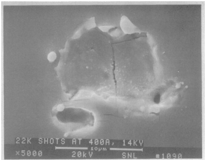
Figure 7. High magnification SEM picture of switch 5. Note that there is damage whose characteristic size is 10 \mu\text{m} and may exhibit melting.
