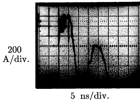
Figure 4. The current through a lock-on switch charged to 75 kV, triggered by a 166 W laser diode array. The scales are 200 A/div. and 5 ns/div. The peak current is 1200 A. The power delivered to an ideal 30 \Omega load would be 40 MW.
