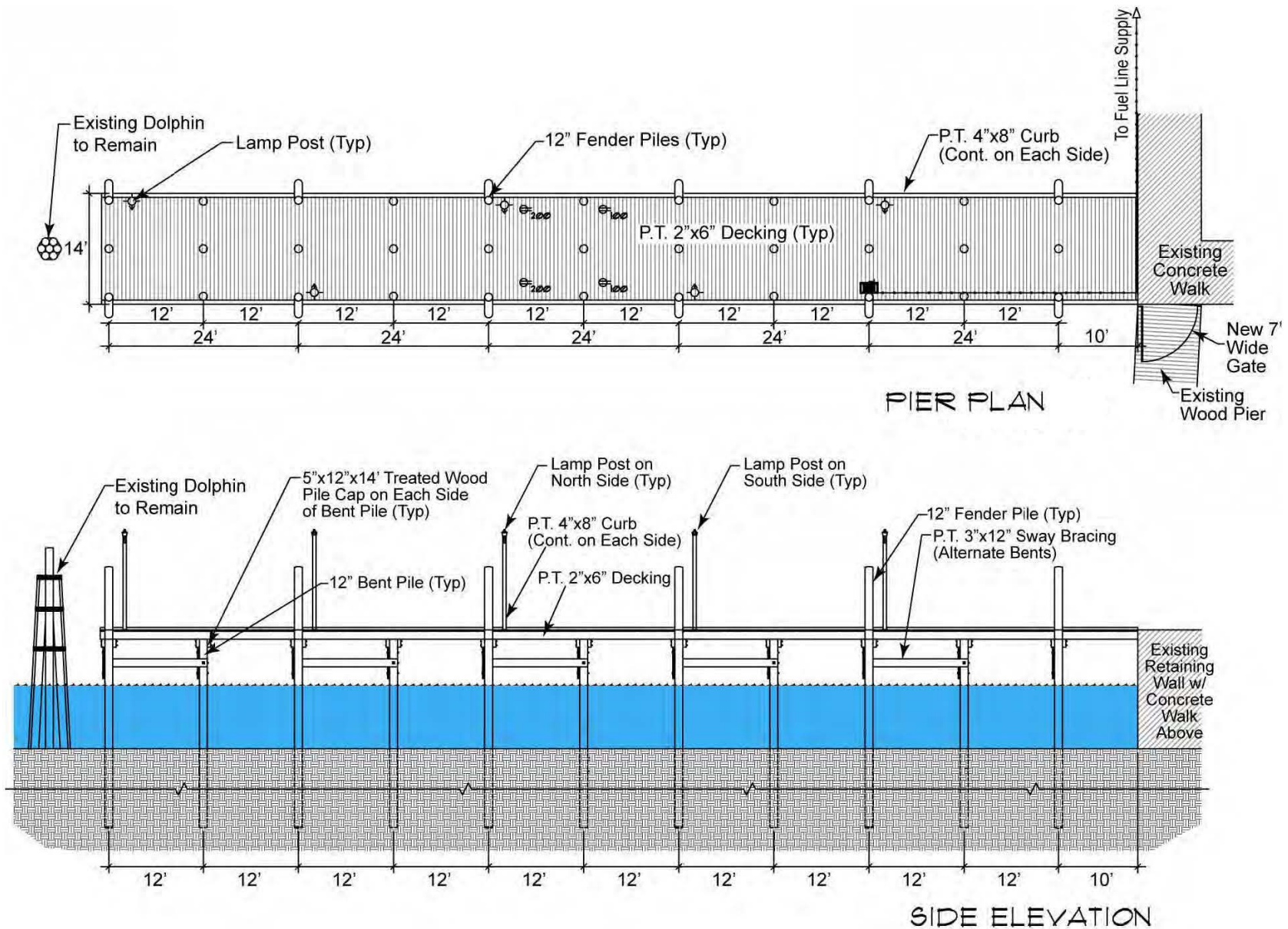
FIGURE 2-7 Preliminary Design Plan and Side Elevation of Proposed Drone Recovery Dock EA for Replacement of Drone Recovery Dock at Tyndall AFB
