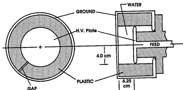
Figure 3. Module used to test the PFA concept
