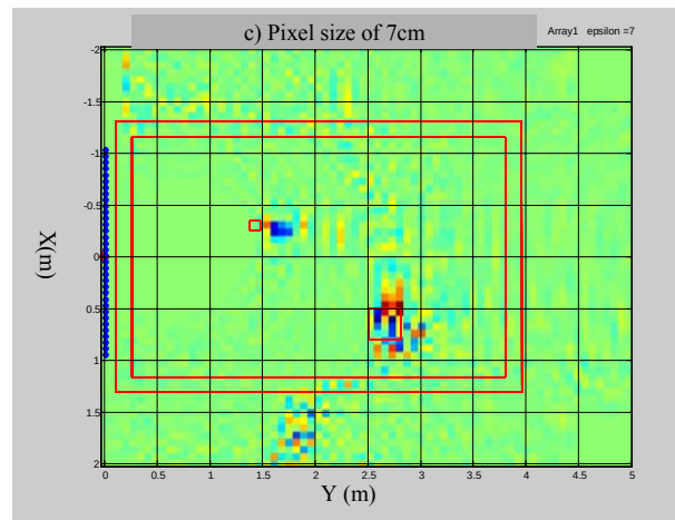
Figure 30. Moving targets: pixel size 1, 3.5, 7 and 10cm
