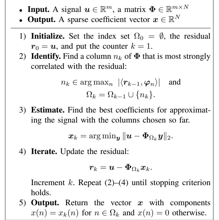
Fig. 1. Orthogonal Matching Pursuit (OMP)
