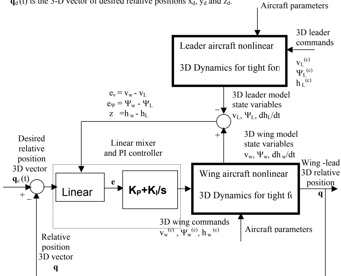
Fig. 3.19 Block diagram for the PI control of the relative distance between two aircrafts in tight formation flight
