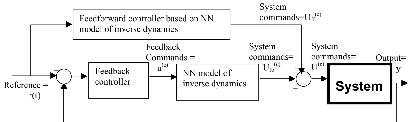
Fig. 3.4 Generic block diagram of a controller using Neural Networks (NN)
