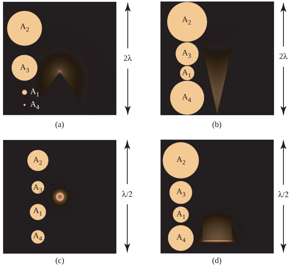
Figure 2. Distributions of (a) \sqrt{W(\mathbf{r})} of WPP mode for \theta = 70^\circ and \rho_{\text{tip}} = 5 \text{ nm} [8]; (b) W(\mathbf{r}) of CPP modes for \theta = 25^\circ and \rho_{\text{tip}} = 5 \text{ nm} ; (c) W(\mathbf{r}) of CyPP modes for d = 50 \text{ nm} ; and (d) W(\mathbf{r}) of HPP mode for a = 200 \text{ nm} and h = 5 \text{ nm} . The discs within each panel show the effective size of the mode using the four measures, A_1 , A_2 , A_3 and A_4 . Note that the plot regions of (a) and (b) are 4\times larger than (c) and (d) and so the discs within these panels must be scaled accordingly. In each plot, \lambda = 1550 \text{ nm} is the vacuum wavelength. The scale of each plot is displayed in units of the vacuum wavelength, \lambda = 1550 \text{ nm} .
