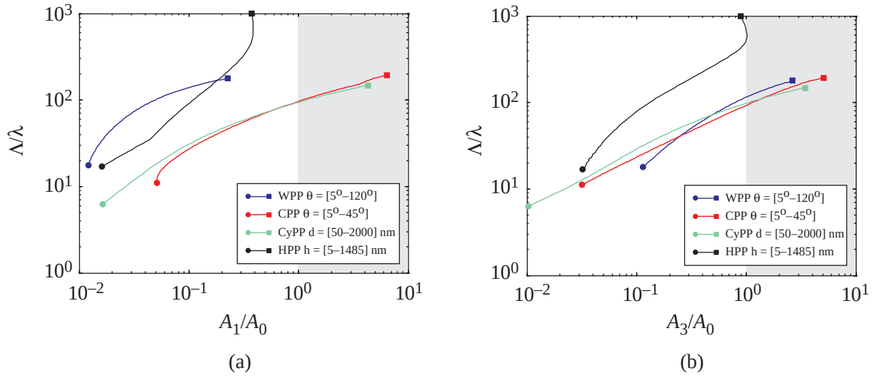
Figure 3. Parametric plots of normalized propagation distance \Delta\lambda and normalized effective mode area: (a) A_1/A_0 and (b) A_3/A_0 . A similar trend results when considering the A_2 measure of mode area; however, A_2 does not represent the same proportion of mode energy for WPPs when compared with the other waveguides (for a comparison of A_2 and A_3 , please see appendix B.)
