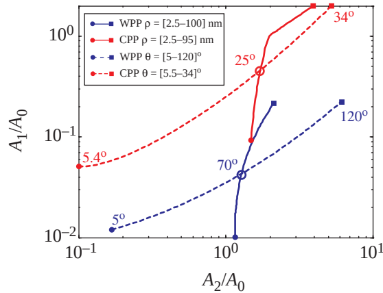
Figure B.2. Comparison of effective mode area, A_1 and A_2 in CPP and WPP waveguides parameterized by the tip radius, \rho (solid lines). Broken lines show the same comparison for \rho = 10 nm parameterized by the sidewall angle, \theta .
