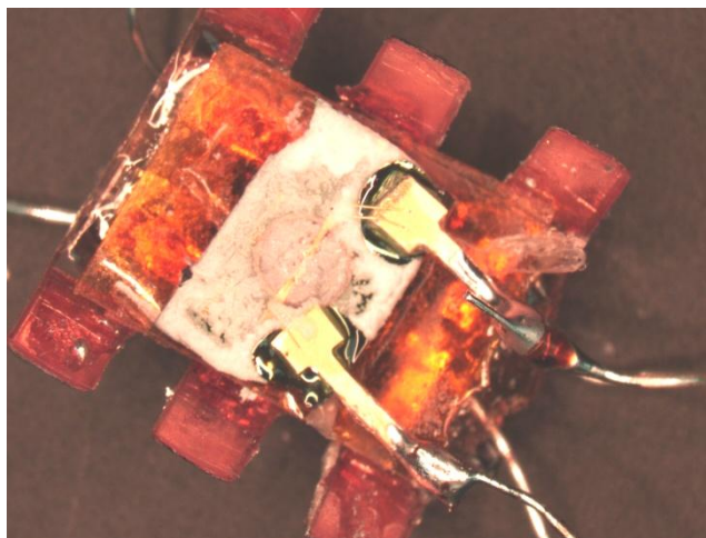
Figure 47 Circuit connected to oxidized nanoporous Si by soldering to pads on the substrate
