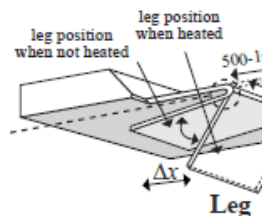
Figure 12 Silicon microrobot with polyimide joint actuators
