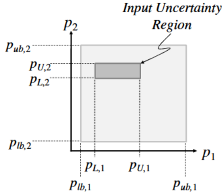
Figure 6.2: Input Uncertainty Region
