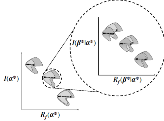
Figure 5.7: Sample Propagation of DISA Result
