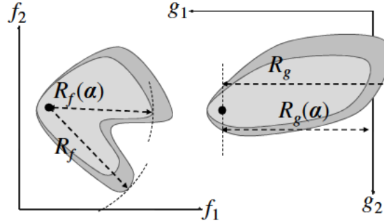
Figure 5.4: Graphical Depiction of R_f(\alpha) and R_g(\alpha)
