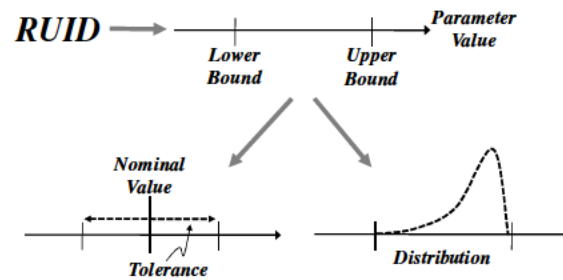
Figure 6.1: Unknown Uncertainty Quantification
