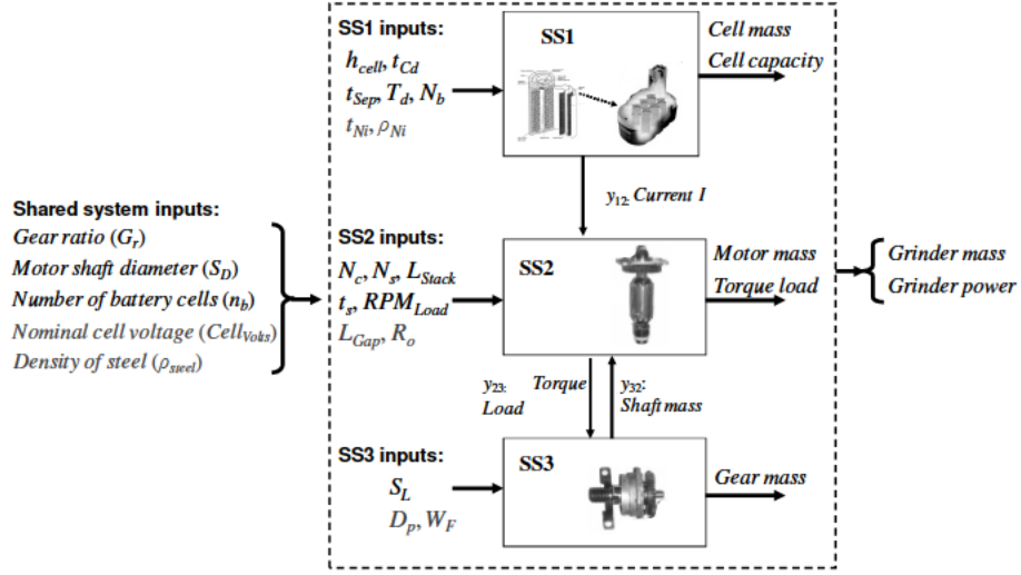
Figure 3.11: Design Variables, Couplings, and Outputs in Grinder Example
