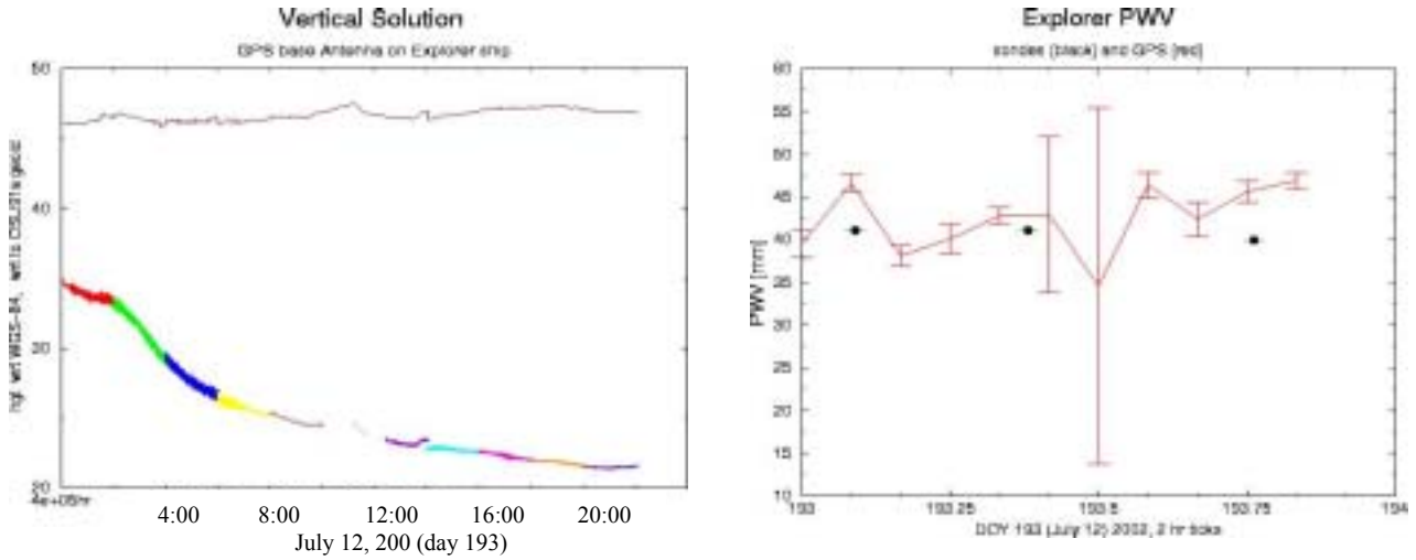
Figure 3 Left panel shows the ellipsoidal height of the ship during day 193. The top curve in the left panel shows the mean sea level height of the "Zephyr" GPS antenna after correction by use of the OSU-91 geoid. The right panel compares GPS estimates of precipitable water vapor (PWV) aboard the ship (red line with vertical error bars representing the formal error of the GPS PWV estimation) with PWV computed from ship-launched radiosondes. (See text for more details)
