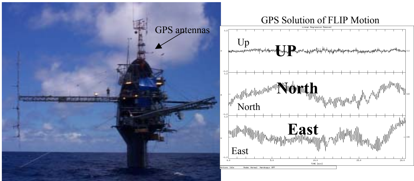
Figure 1 (left panel) shows the location of the GPS antennas on the Flip ship during the experiment. The right panel shows an example 20-minute segment of the GPS-determined motion of Flip after removal of a linear trend for the up, north and east motion components. The scale in each of the motion panels is \pm 1.2 m. The period of the primarily north and east motion is about 10-sec.
