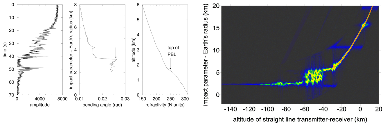
Figure 4 . The three small panels on the left show signal amplitude (left), signal bending (middle), and retrieved refractivity for a RO occultation from the CHAMP satellite. A sharp refractivity gradient indicating the PBL can be seen at \sim 1.7 km. The right panel is a sliding spectrogram of a simulated RO signal based on a high-resolution radiosonde, which indicated super refraction layers. The horizontal lines of constant ray asymptote (which is the same as impact parameter minus Earth radius) can be used to identify the super refraction layers. The lowest one in these simulations is at 200 meters above the surface. (See text for more details)
