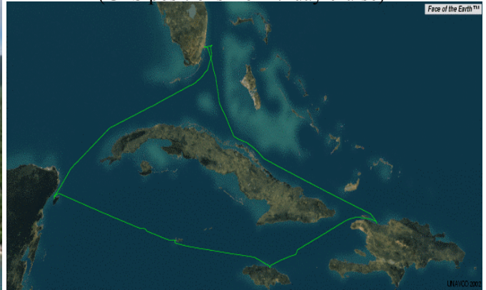
Caribbean track of the "Explorer of the Seas" (GPS positions from 7-day cruise)
