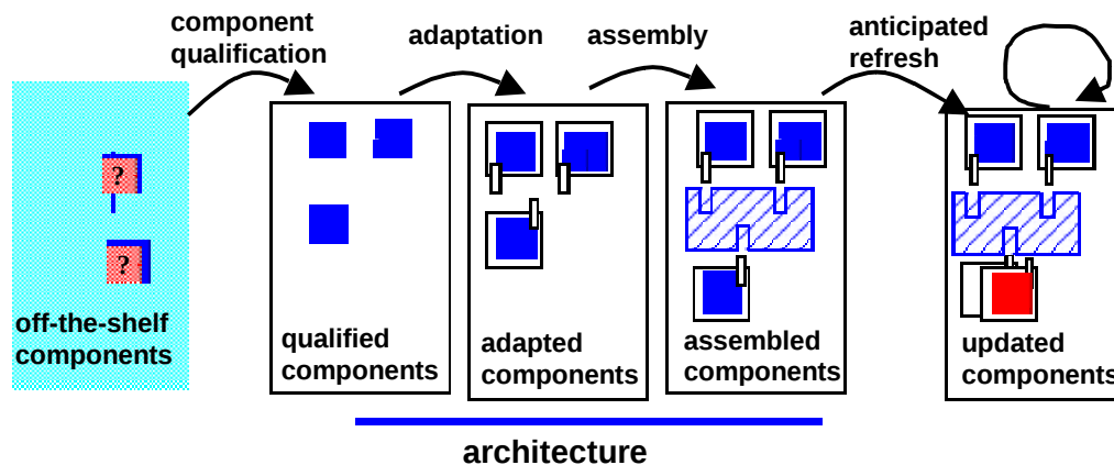
Figure 1: Creating COTS-Based Systems
