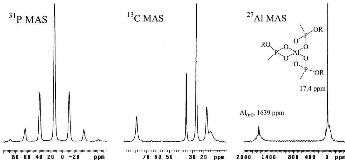
Figure 5. ^{31}\text{P} , ^{13}\text{C} , and ^{27}\text{Al} MAS NMR spectra obtained at 7.0 T for GD reacted with \text{Al}_{(\text{m})} in the presence of water. Insets show assignments of peaks to \text{Al}_{(\text{m})} and aluminophosphonate 1 (see text).
