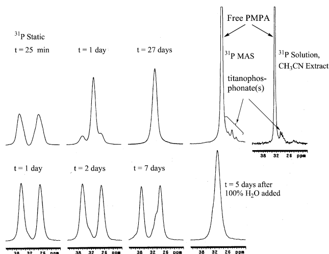
Figure 6. Selected ^{31}\text{P} and ^{31}\text{P} MAS NMR spectra obtained for GD reactions with anatase (11 wt % water added; top spectra) and rutile (bottom spectra; before and after 100 wt % water added).
